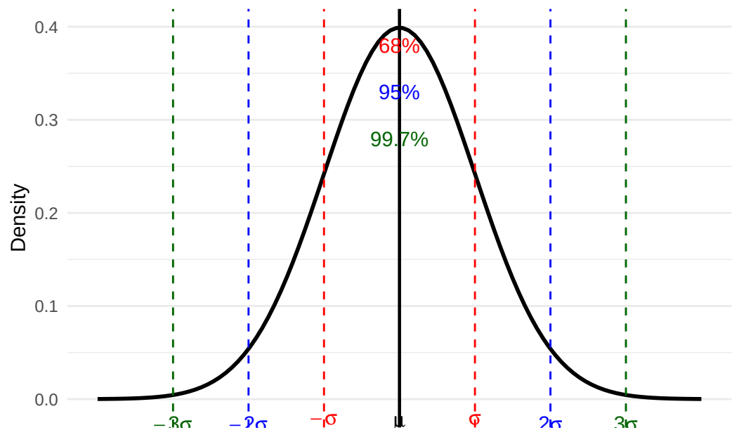
Normal Distribution with 68–95–99.7 Rule
