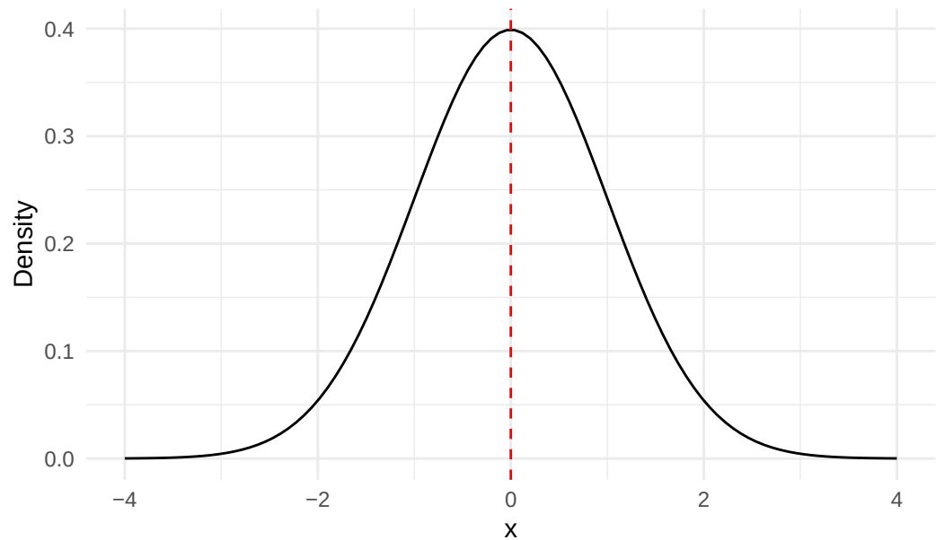
Normal Distribution N(0,1)
