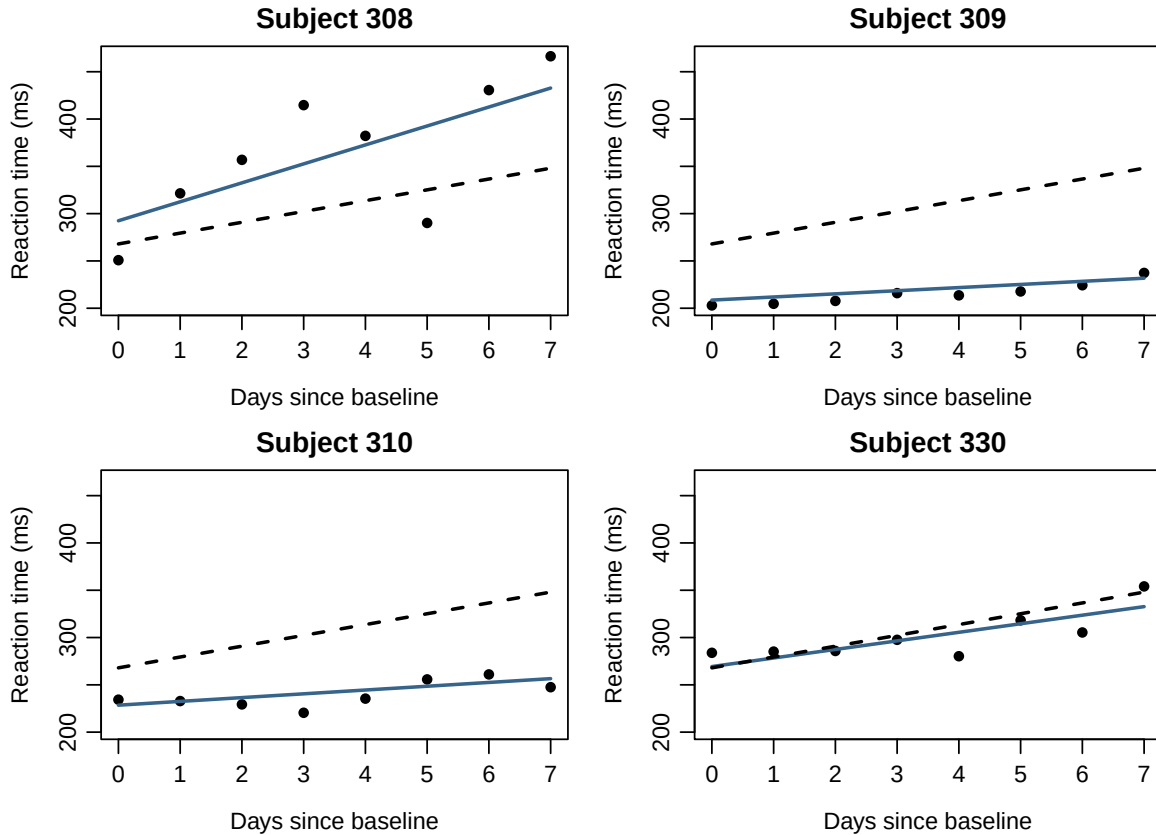
Figure 11.6: Four subjects from the sleepstudy data. Blue lines include each subject's fitted random effects; dashed lines use only the common fixed effects. A common linear trend does not require identical subject trajectories.
