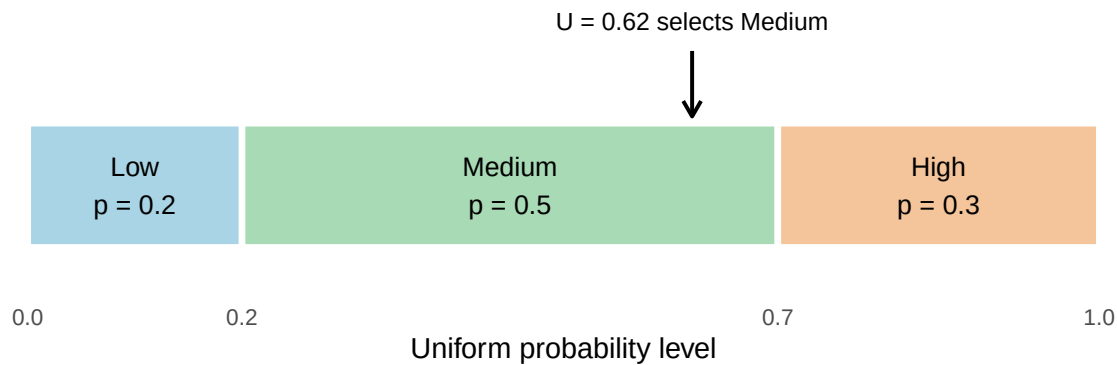
Figure 4.3: Discrete generation allocates the unit interval to outcomes. The middle category receives half of the interval, so it is selected with probability 0.5. Boundary points follow the generalized-inverse convention and have probability zero for an ideal continuous uniform.
