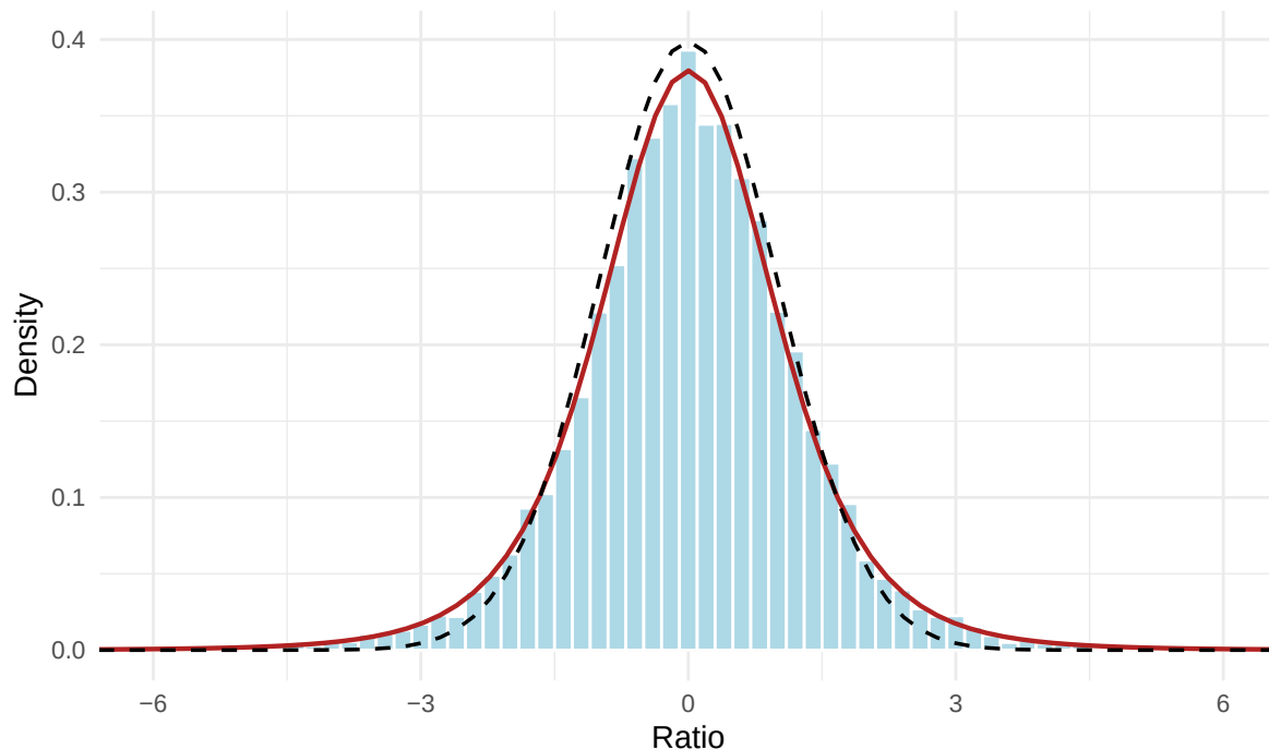
Figure 4.6: A random denominator creates heavier tails. The generated ratios agree with the t distribution with 5 degrees of freedom; the dashed normal density has lighter tails.
