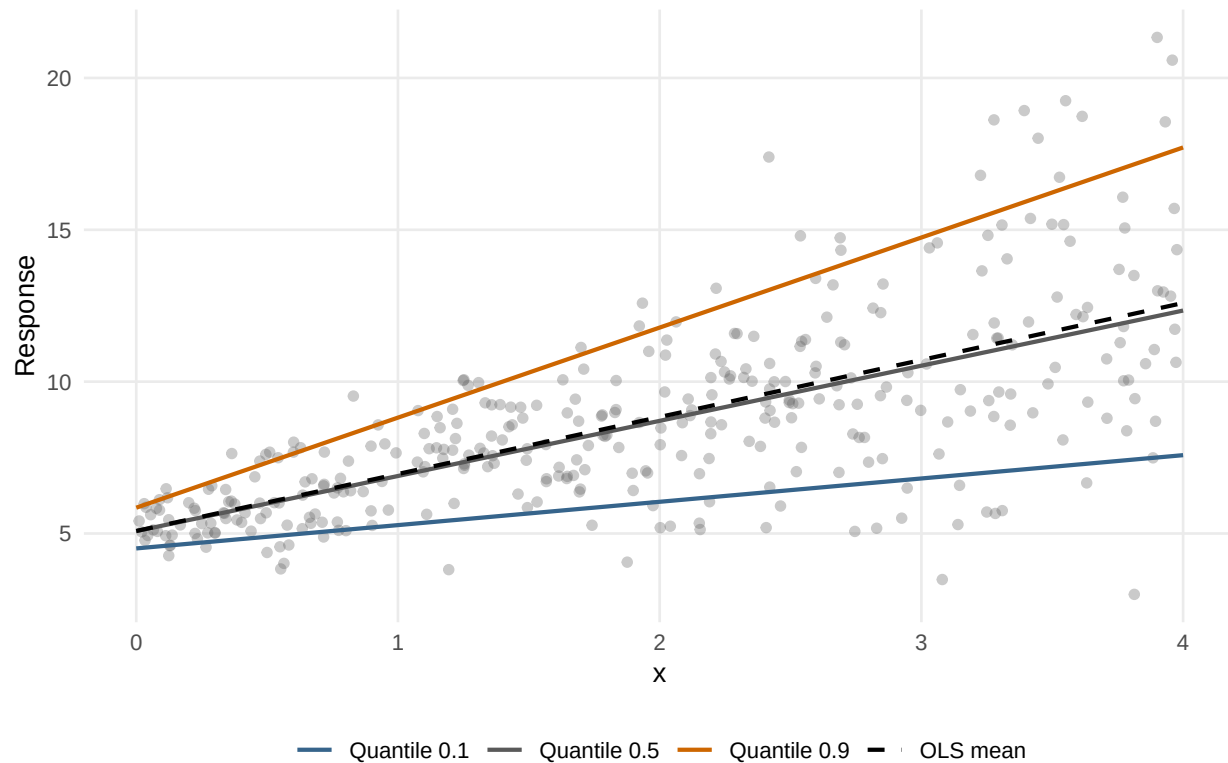
Figure 5.4: Fitted conditional quantiles and the OLS mean in simulated data with increasing spread. The growing distance between the lower and upper quantiles reveals variation that a mean line alone does not describe.
