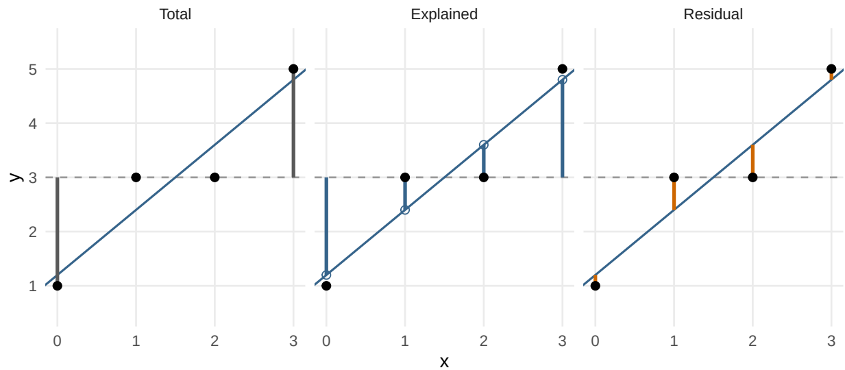
Figure 4.2: Total deviations from the sample mean, explained deviations of fitted values from the mean, and residual deviations from the fitted line. SST = SSR + SSE holds after summing across observations; it is not a point-by-point identity between squared deviations.
