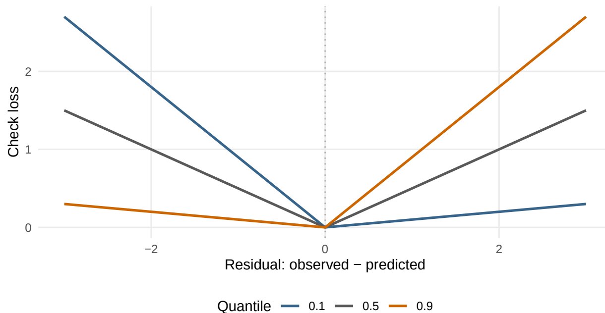
Figure 5.3: Check loss for three quantiles. A positive residual means the prediction is too low. The upper-quantile loss penalizes that side more strongly.
