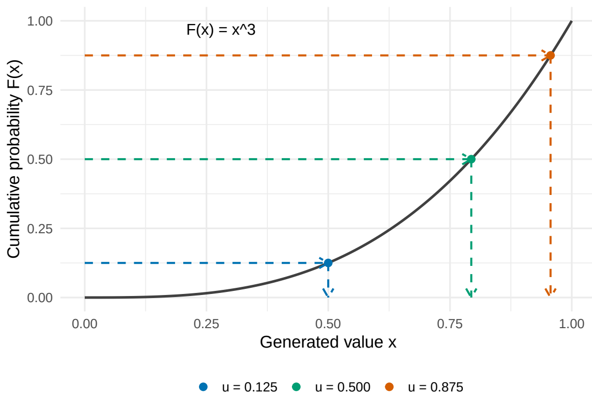
Figure 4.1: The inverse CDF converts a probability level into an observation. Each horizontal arrow starts at u ; the downward arrow lands at x = \sqrt[3]{u} . The dashed guides are a construction, not additional random draws.
