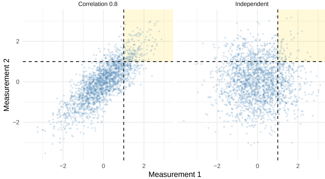
Figure 4.10: The marginal distributions are the same in both panels. Positive correlation puts more probability in the upper-right region where both measurements exceed 1.
