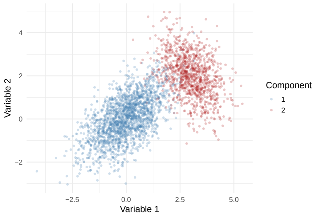
Figure 4.11: Each point is generated from one bivariate normal component. The label determines both its coordinates and its covariance structure.
