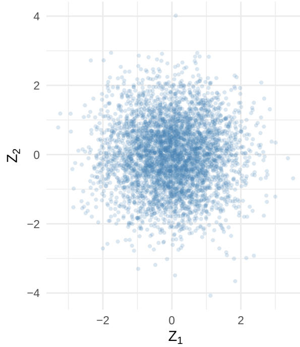
Figure 4.5: Box-Muller creates a circular normal cloud from two independent uniforms. The two normal coordinates are independent even though their formulas share a radius and angle.
