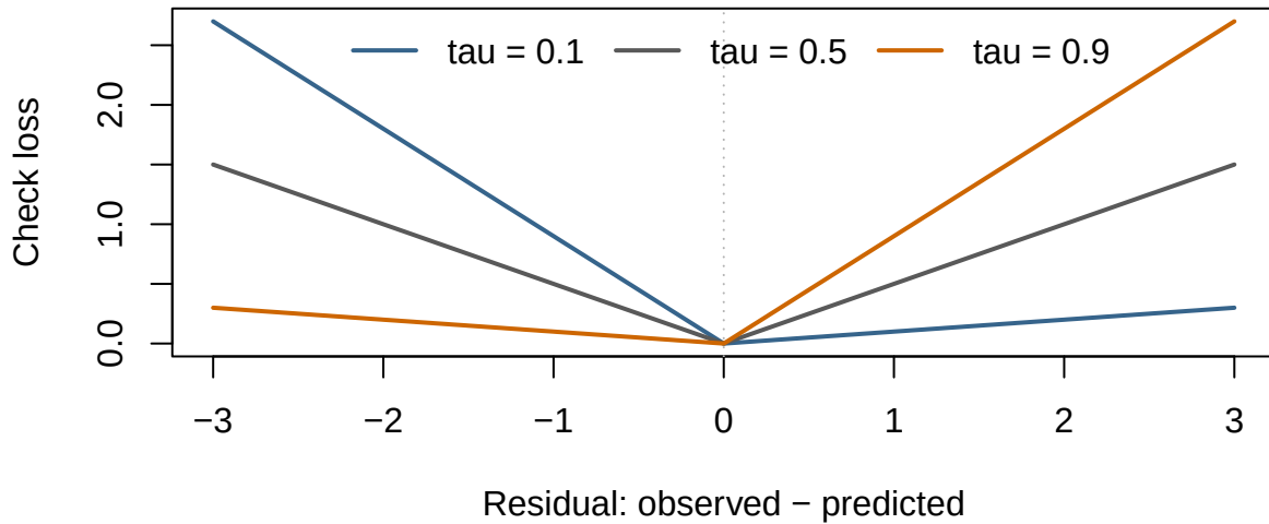
Figure F.1: Check loss for three quantiles. A positive residual means the prediction is too low. The upper-quantile loss penalizes that side more strongly.
