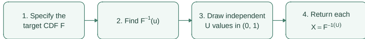
Figure 4.1: Inverse transformation: prepare one map, then apply it to independent uniforms.
