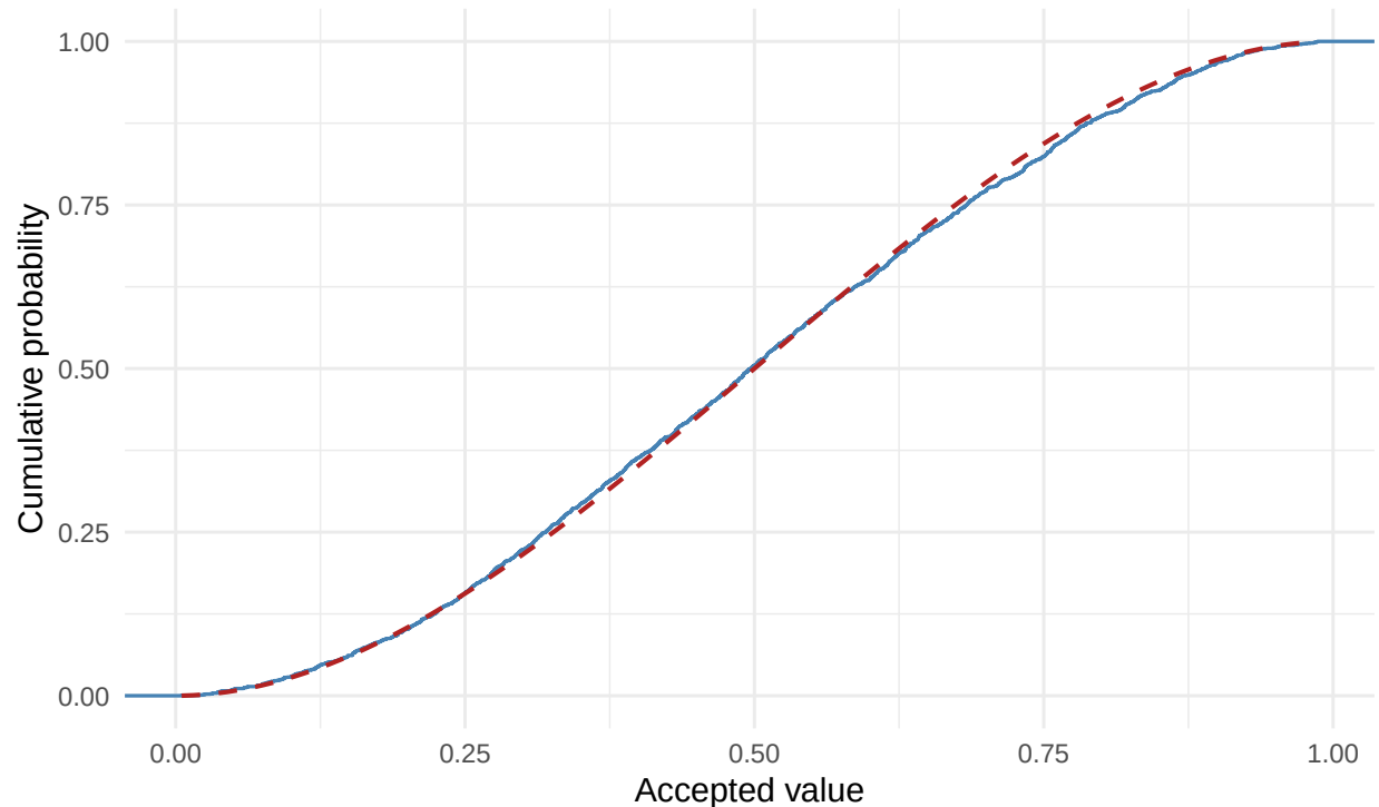
Figure 4.17: The empirical CDF of accepted proposals tracks the Beta(2,2) CDF. Sampling variation creates small discrepancies even for a correct generator.
