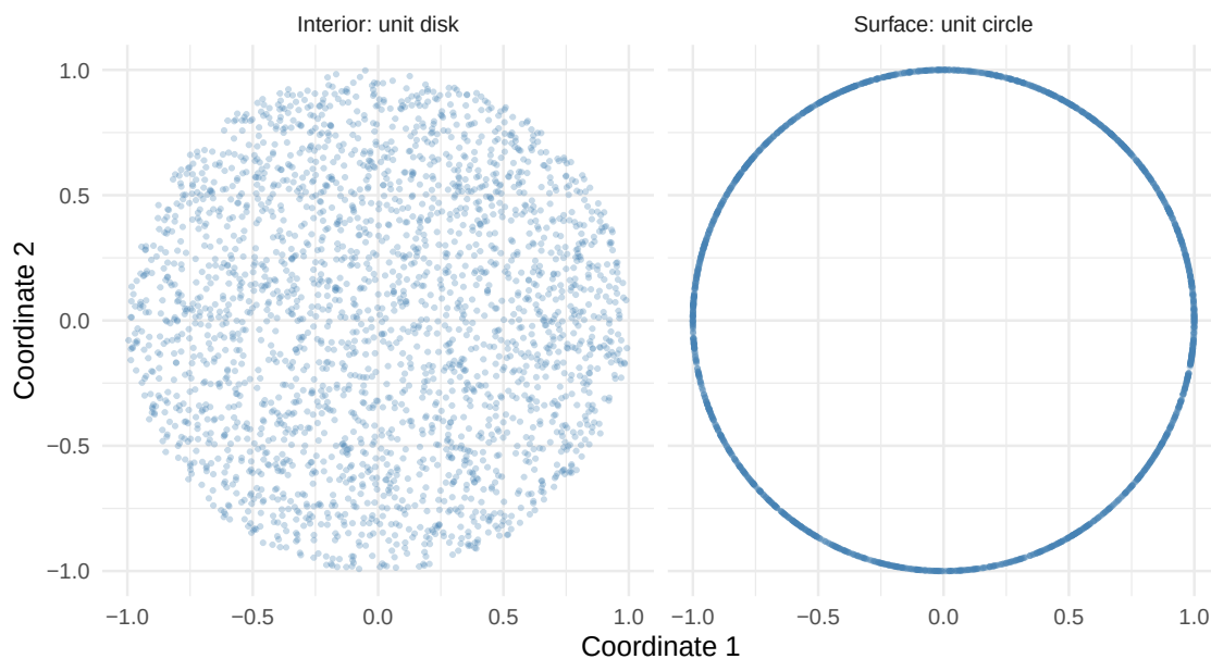
Figure 4.16: In two dimensions, normalized normals lie on the circle. Multiplying by an independent square-root-uniform radius fills the disk uniformly in area.
