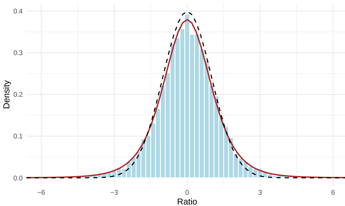
Figure 4.8: A random denominator creates heavier tails. The generated ratios agree with the t distribution with 5 degrees of freedom; the dashed normal density has lighter tails.
