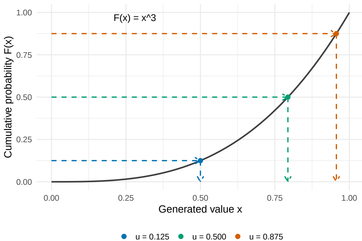
Figure 4.2: The inverse CDF converts a probability level into an observation. Each horizontal arrow starts at u ; the downward arrow lands at x = u^{1/3} . The dashed guides are a construction, not additional random draws.
