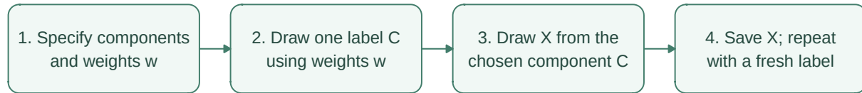
Figure 4.10: A mixture chooses a component before generating an observation.
