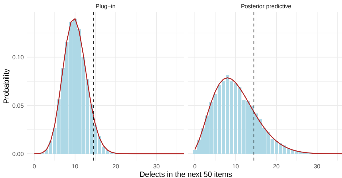
Figure 4.19: The posterior predictive distribution spreads probability over a wider range of defect counts. The plug-in model ignores uncertainty about the process rate. Lines show exact probabilities and bars show simulated proportions.
