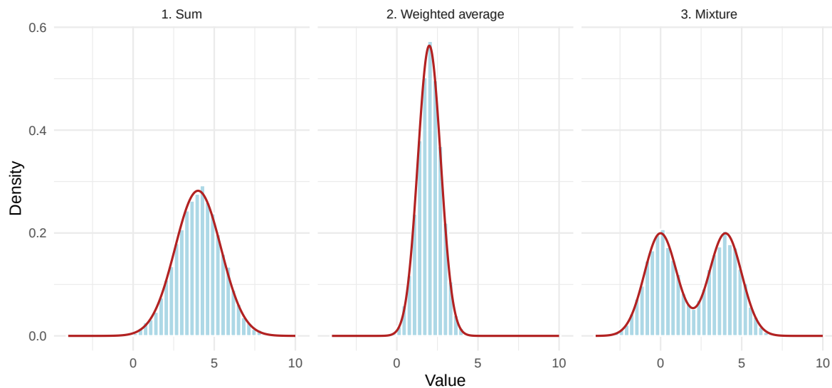
Figure 4.11: Adding two observations, averaging them, and selecting one population produce different distributions. The solid curves show their respective theoretical densities.
