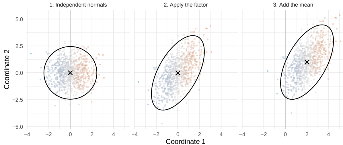
Figure 4.13: A matrix factor introduces scale and dependence; adding the mean shifts location. The black curves are corresponding 95% normal probability contours. All three panels use the same underlying draws and the same axis scale.
