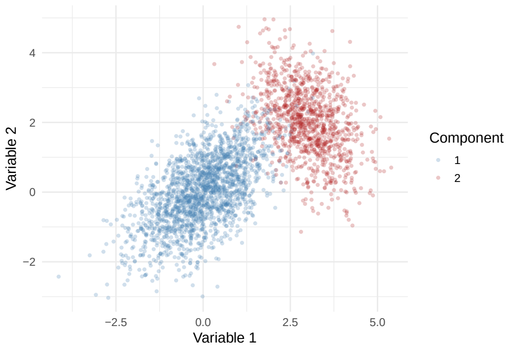
Figure 4.15: Each point is generated from one bivariate normal component. The label determines both its coordinates and its covariance structure.
