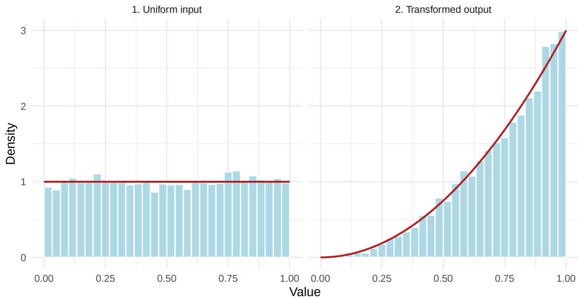
Figure 4.3: Left: uniform probability levels. Right: mapping them through the quantile function produces values with the increasing target density.
