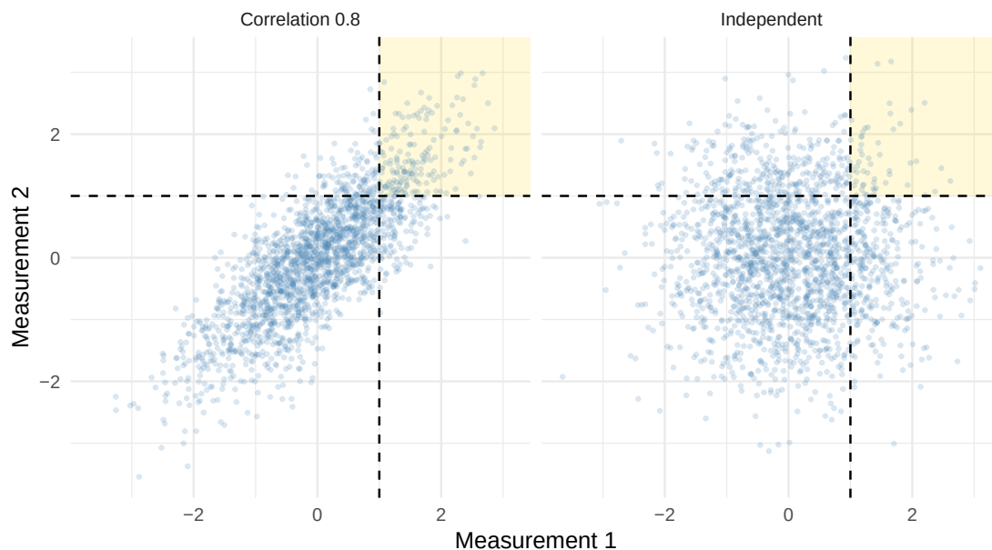
Figure 4.14: The marginal distributions are the same in both panels. Positive correlation puts more probability in the upper-right region where both measurements exceed 1.
