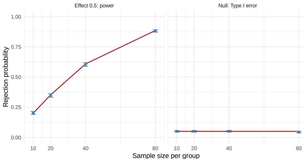
Figure 4.18: Points are simulated rejection rates with approximate 95% Monte Carlo error bars. Lines are exact normal-model probabilities. Increasing the experiment's sample size increases power, while the Type I error remains near 0.05.
