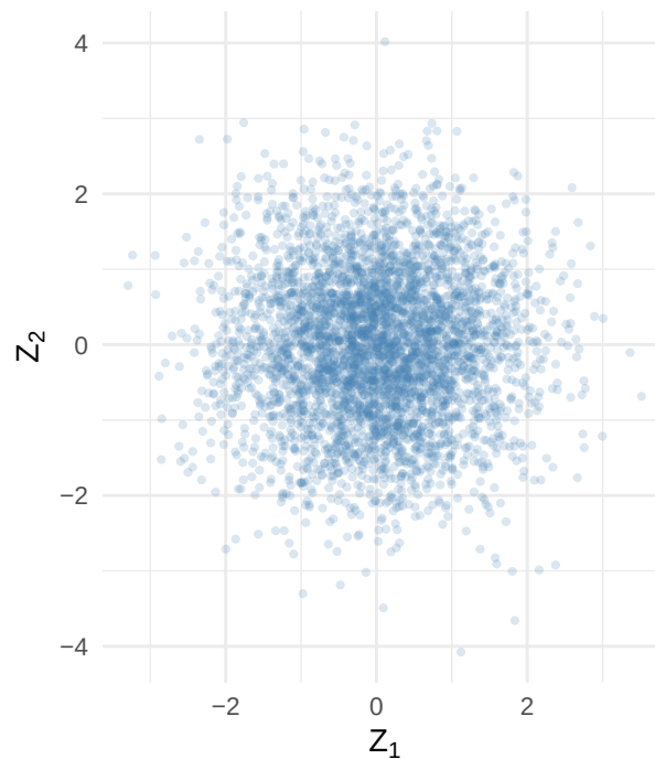
Figure 4.7: Box-Muller creates a circular normal cloud from two independent uniforms. The two normal coordinates are independent even though their formulas share a radius and angle.
