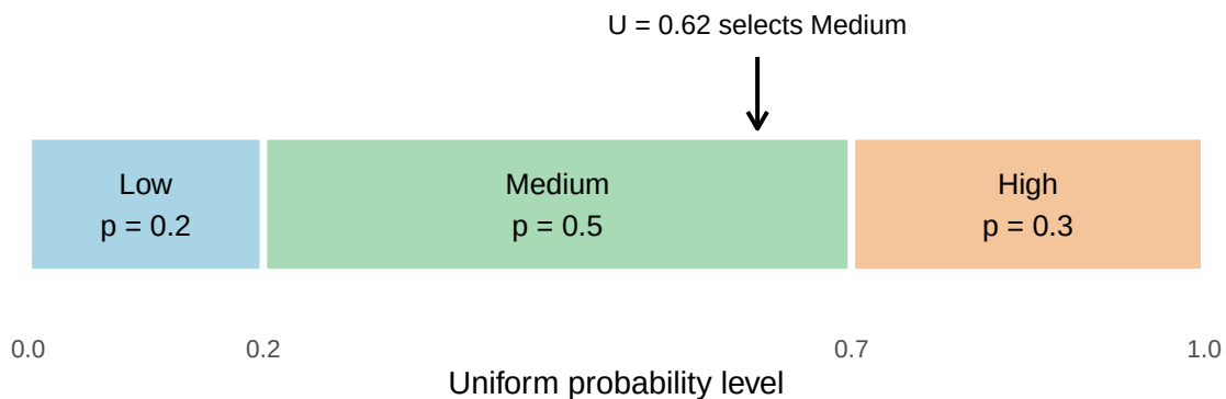
Figure 4.4: Discrete generation allocates the unit interval to outcomes. The middle category receives half of the interval, so it is selected with probability 0.5. Boundary points follow the generalized-inverse convention and have probability zero for an ideal continuous uniform.
