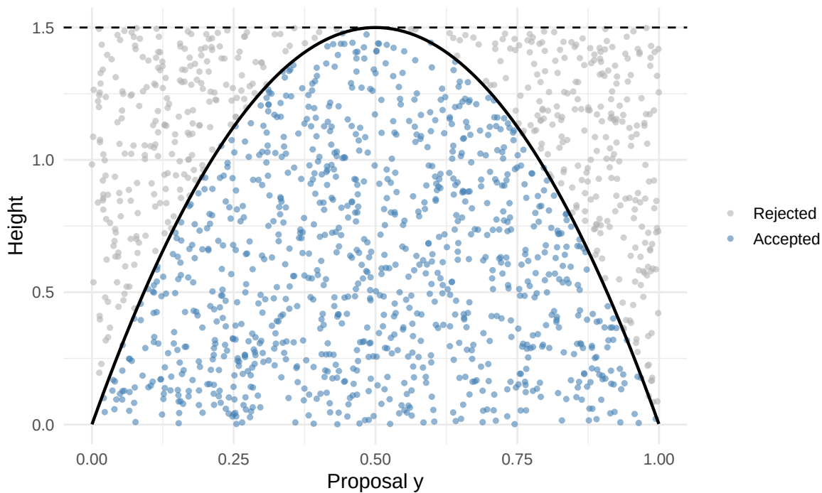
Figure 4.6: Uniform proposals form points under the envelope of height 1.5. Retaining only points below the target density produces Beta(2,2) draws along the horizontal axis.
