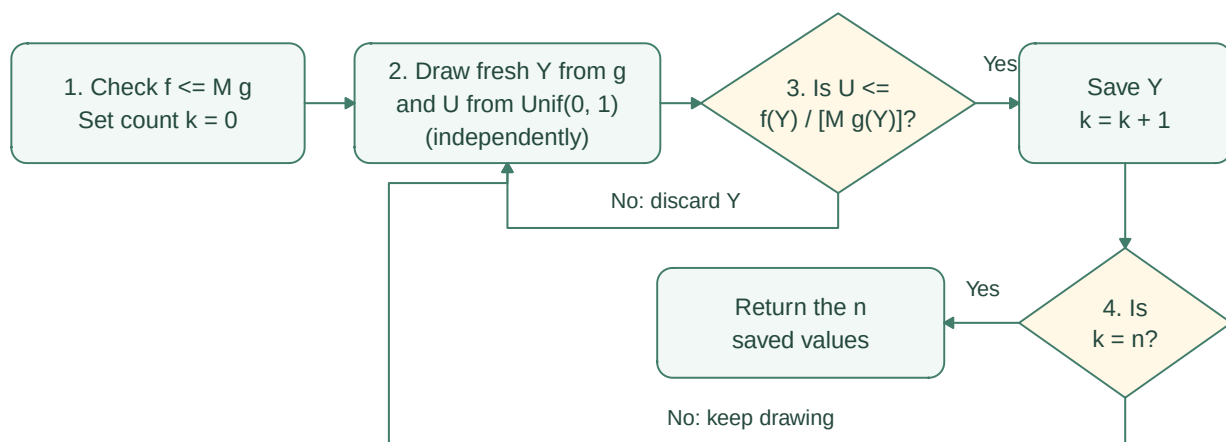
Figure 4.5: Rejection sampling: count accepted values, not attempted proposals.
