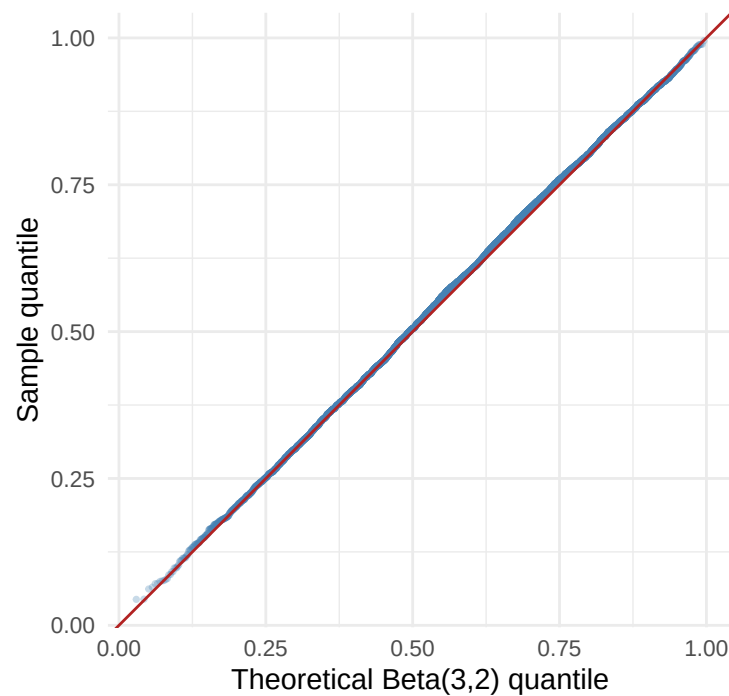
Figure 4.9: A quantile comparison checks the entire distribution of the gamma ratio against Beta(3,2), including its tails.
