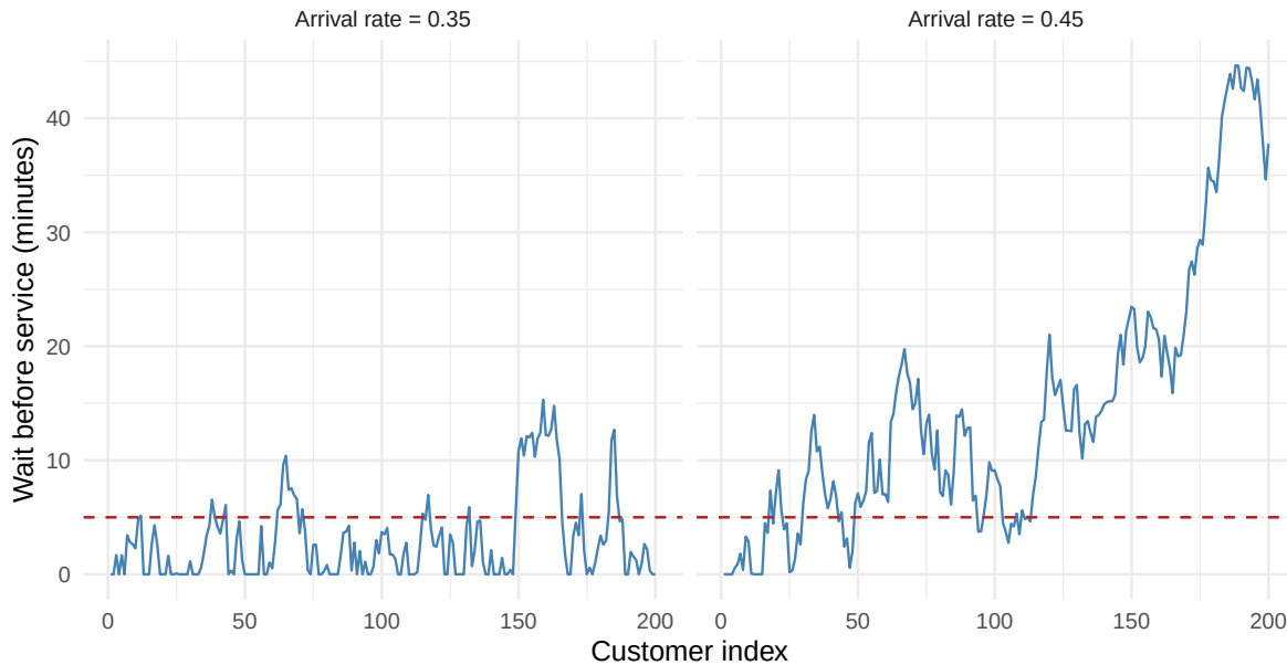
Figure 4.20: Two illustrative paths show how delays carry over between customers. Estimates in the table average 800 independent runs per scenario; one path alone can be misleading.
