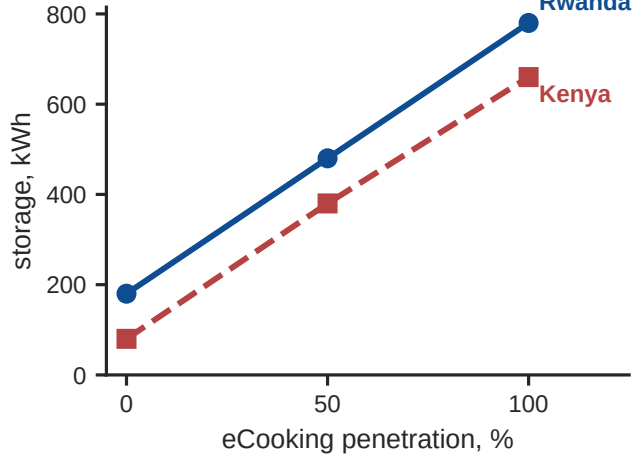
(b) least-cost storage
