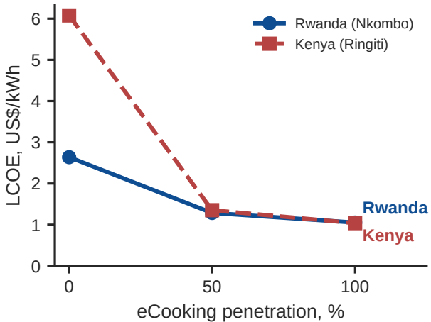
(a) levelised cost
