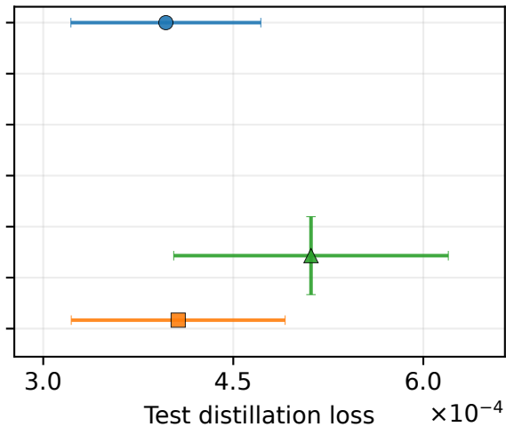
Transformer
