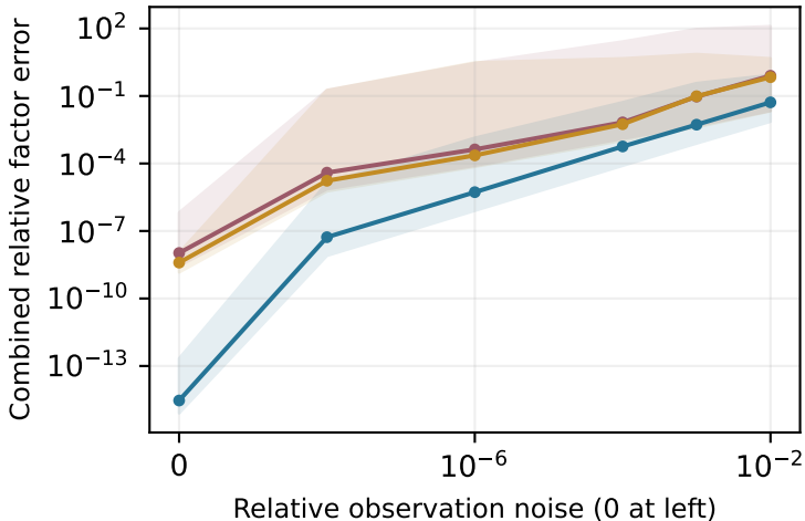
Synthetic: 40 independent seeds
