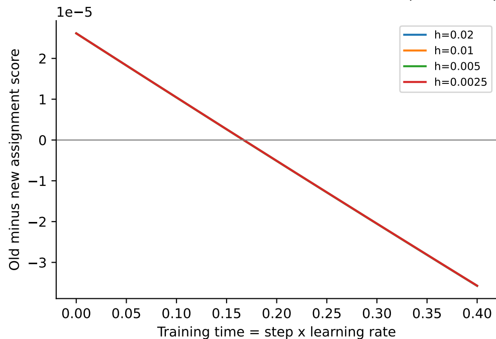
C. Same real trained state + fixed real text (FP64 SGD)
