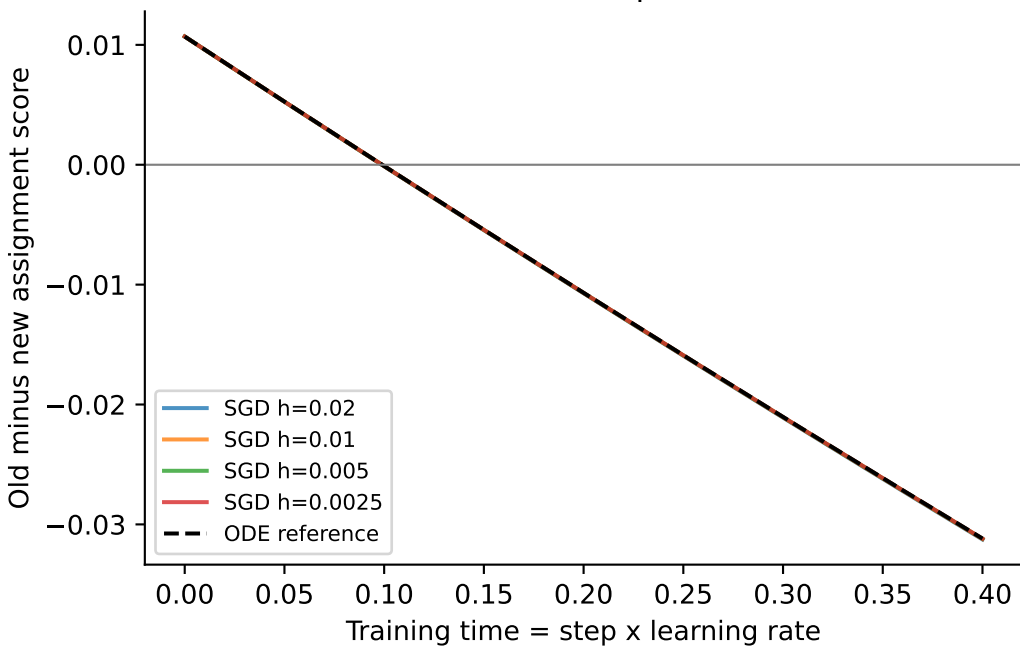
C. Same real trained state + fixed real text (FP64 SGD)
