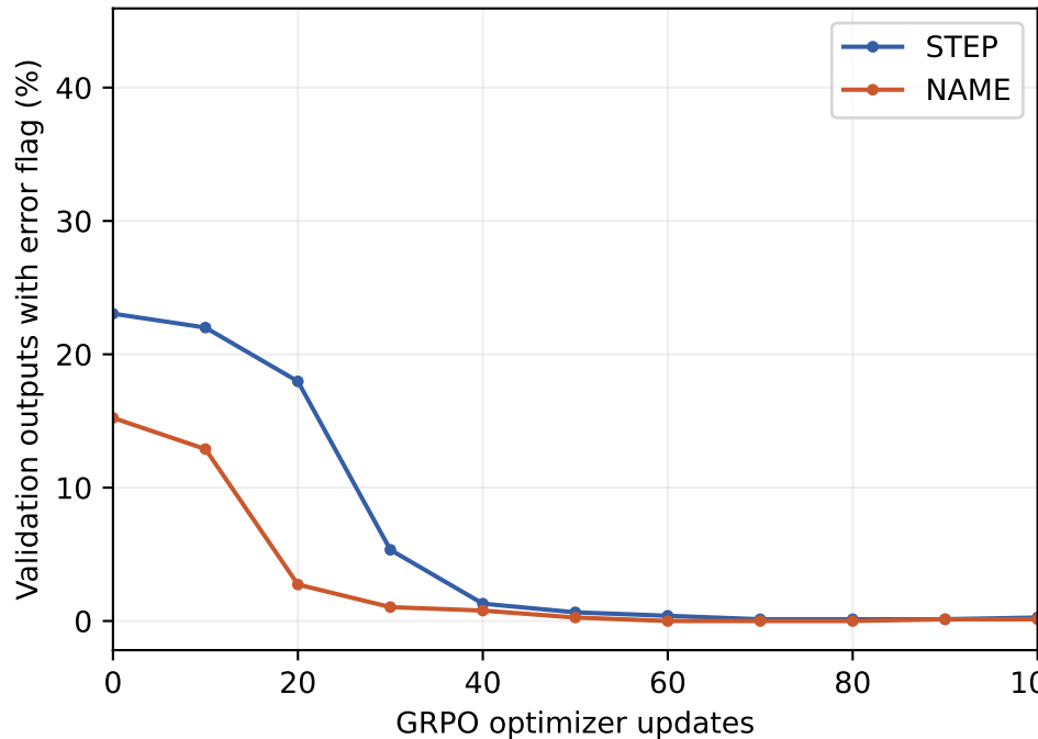
Operation-sequence mismatch
