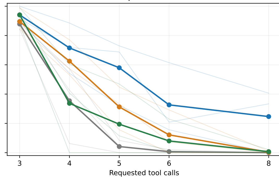
qwen32b
