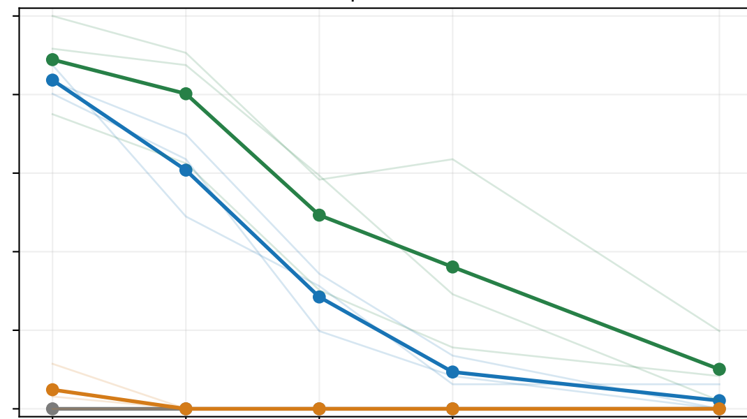
qwen32b
