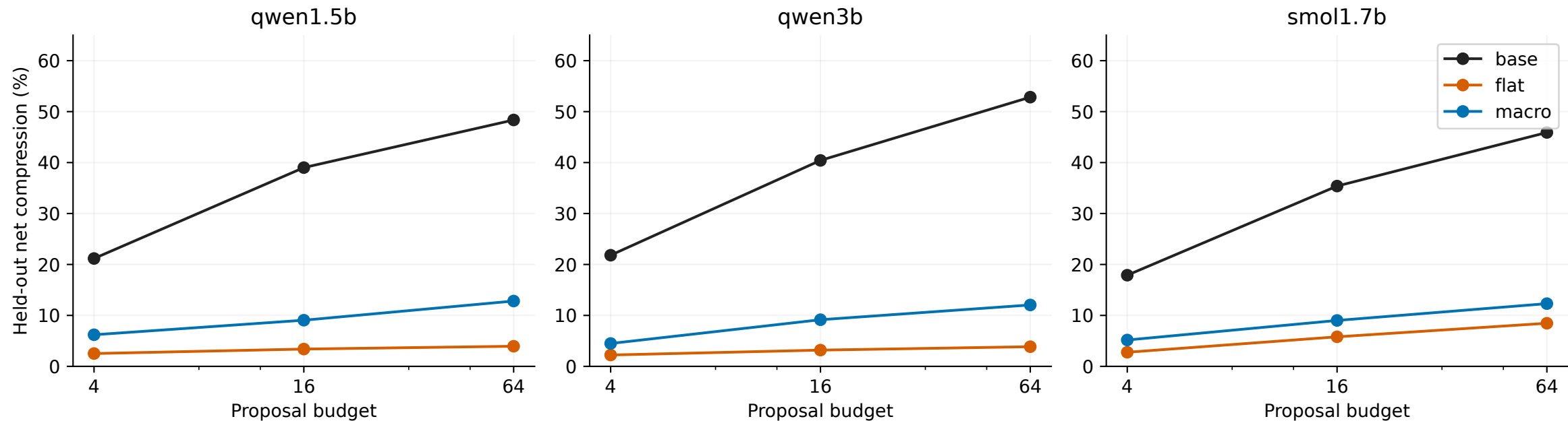
Execution fine-tuning and proposal utility: fixed instruction prompt
