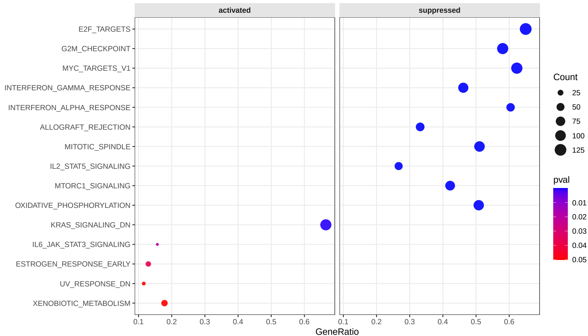
GSEA: T cell – gamma_delta_Th17_like_T_cells vs rest
