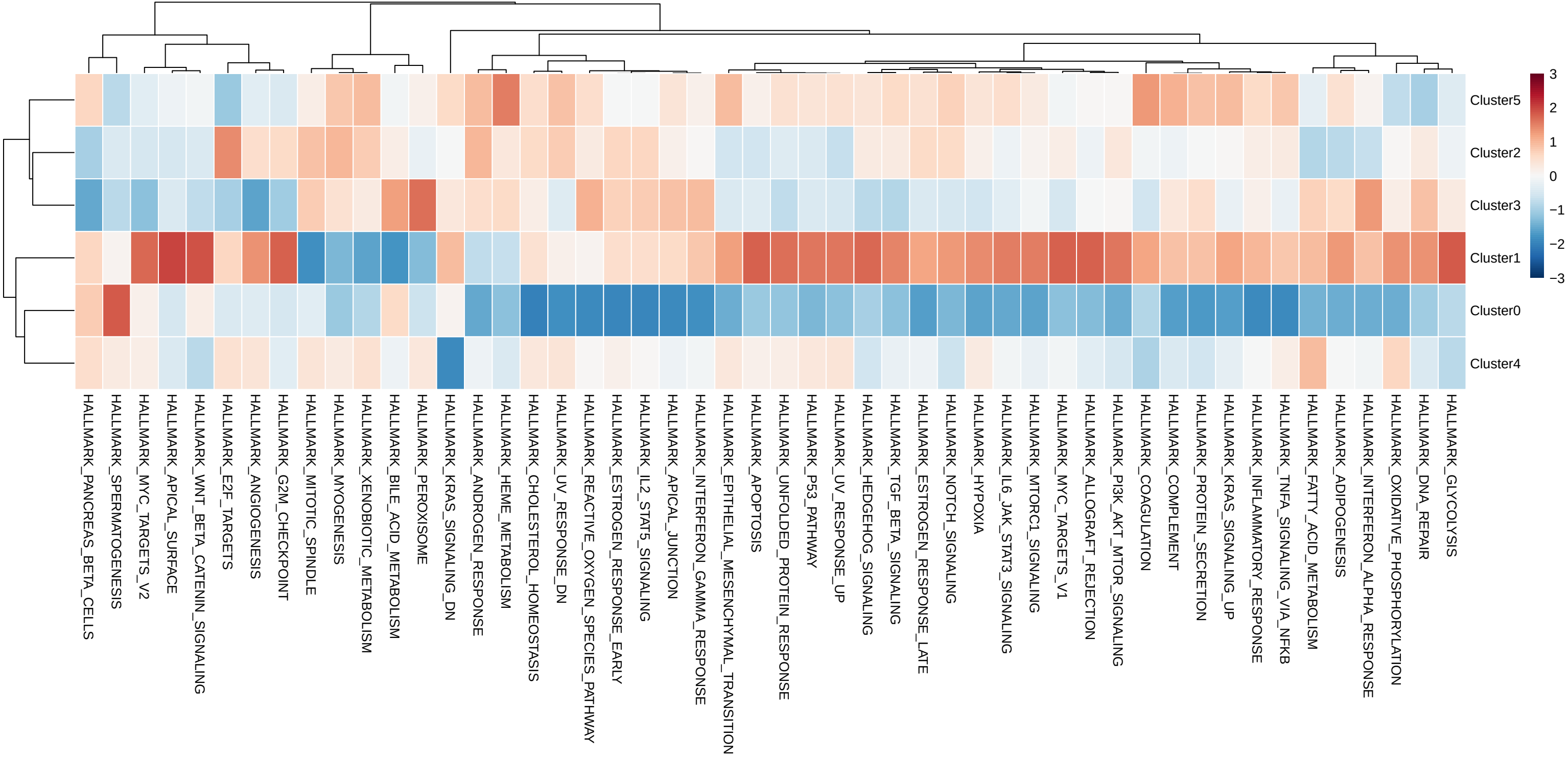
Hallmark Pathway AUCell Activity across DC Subclusters
