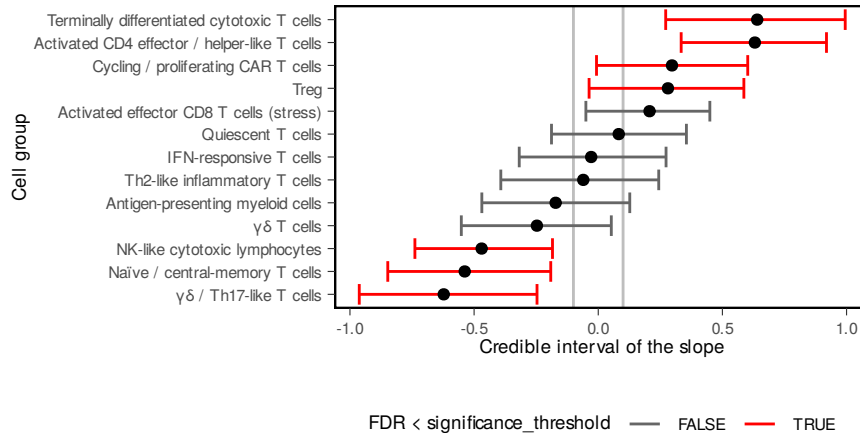
c conditionSTOP
