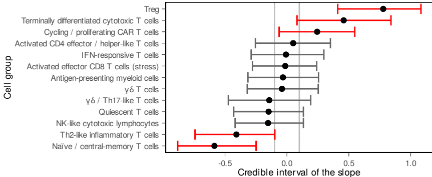
c condition41BB-L
