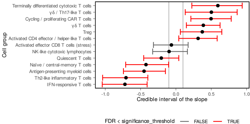
c conditionCD8-41BB
