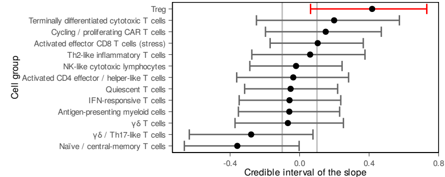
c conditionCD28-41BB
