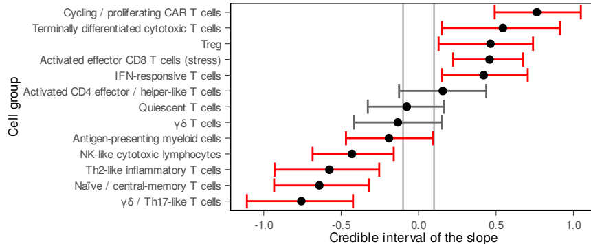
c conditionB7H3
