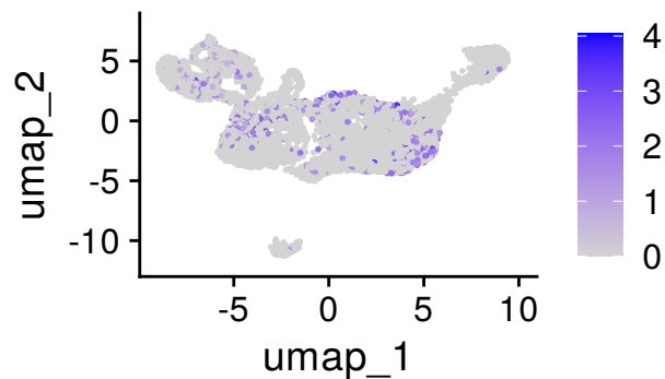
Ccr7
