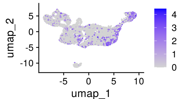
Sell
