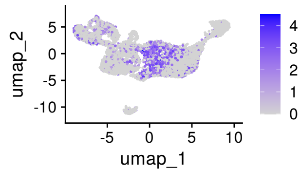
Sell
