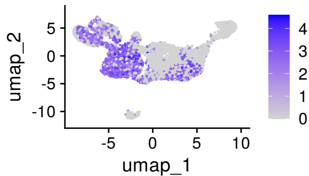
Tcf7
