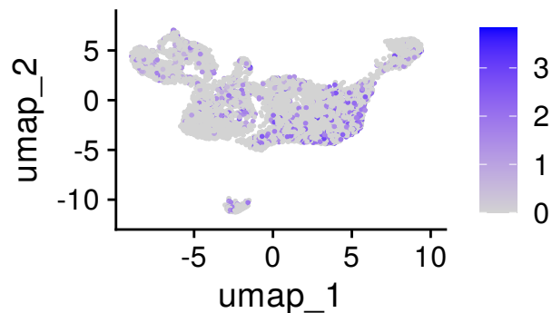
Ccr7
