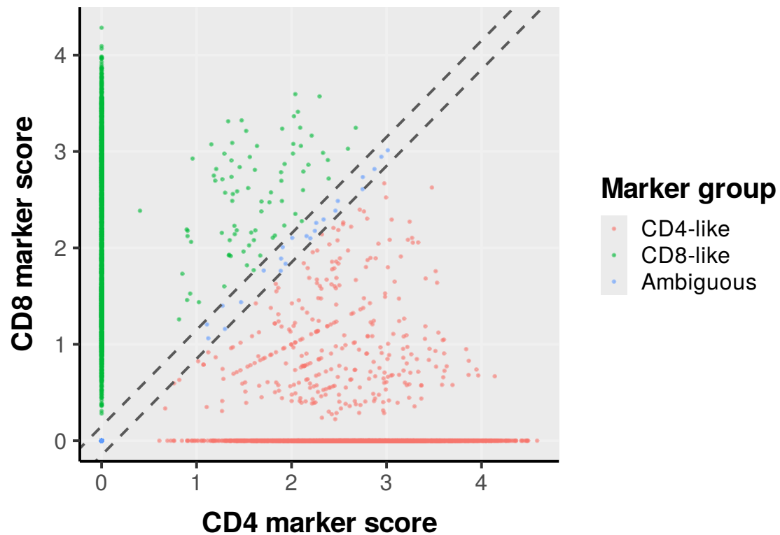
CD4/CD8 marker-score split
