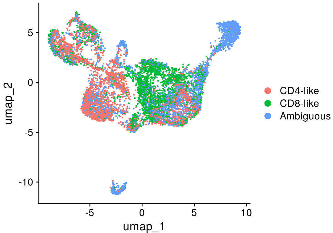
CD4/CD8 marker-based groups
