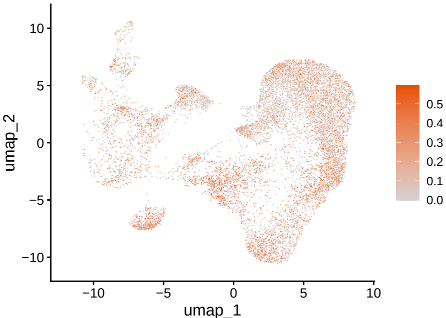
tumor
