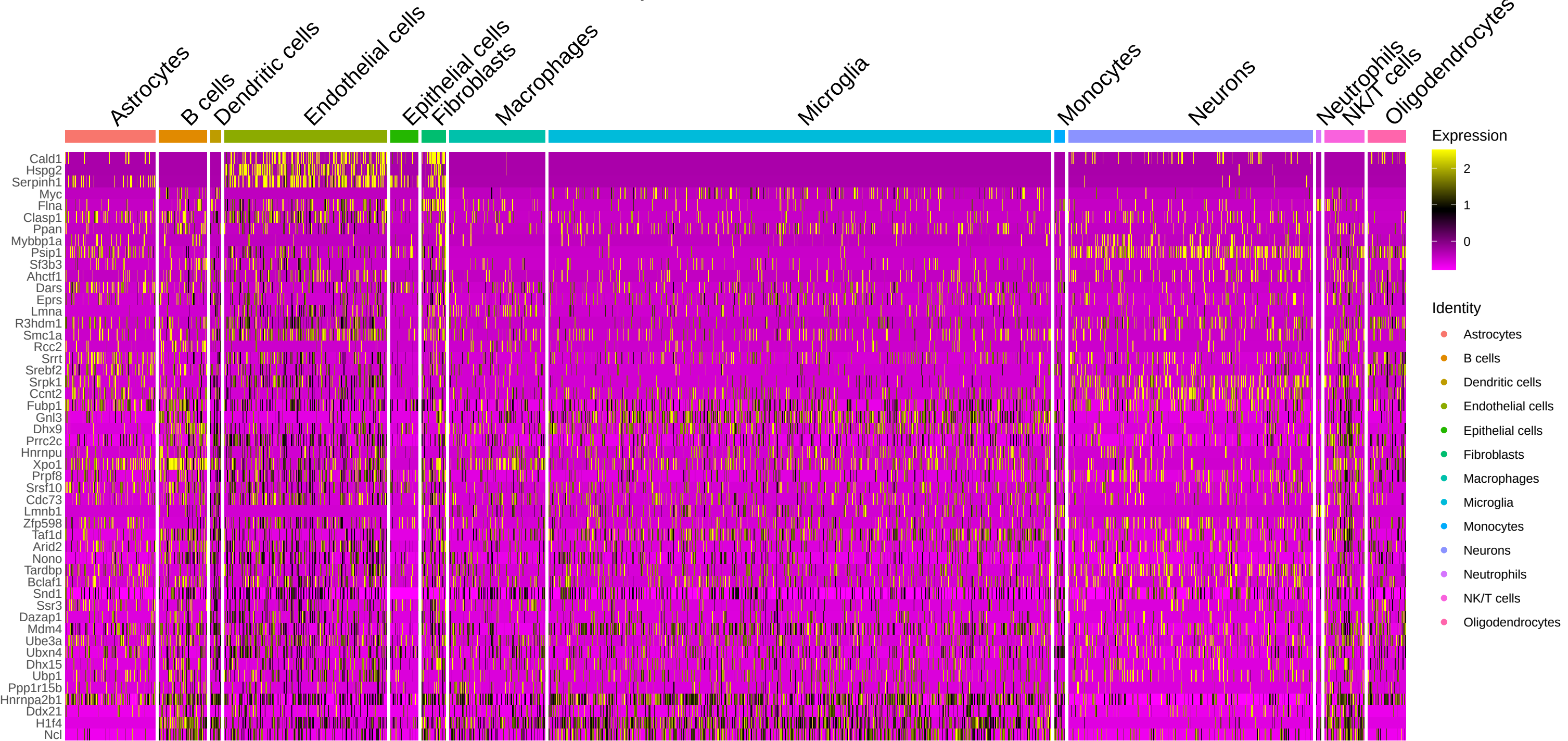
Top Markers for Fibroblasts
