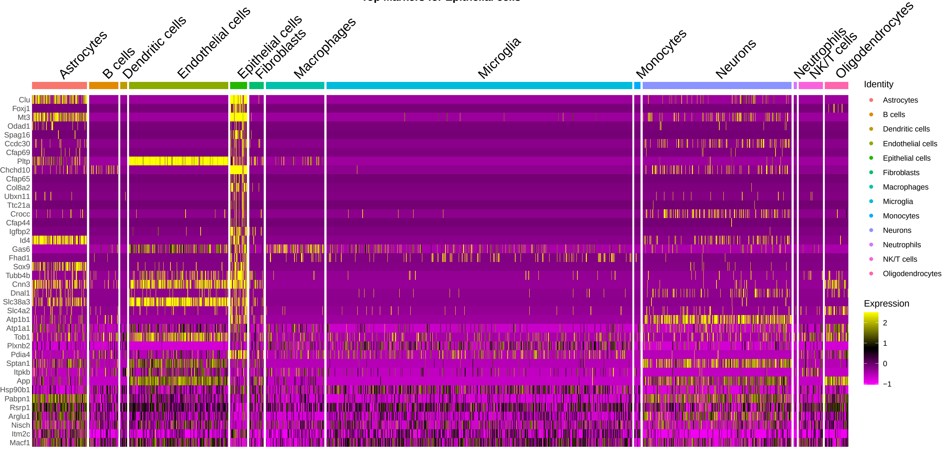
Top Markers for Epithelial cells
