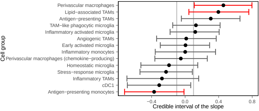
c conditionCD28-41BB
