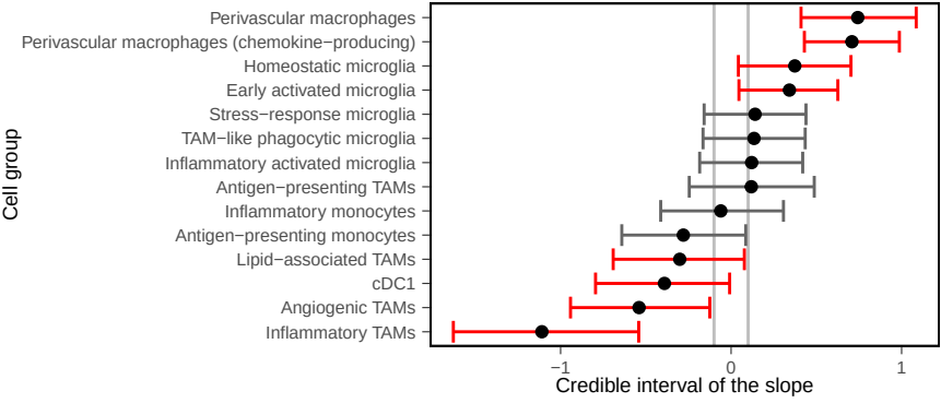
c conditiontumor
