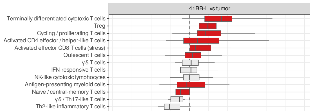
T cell miloR logFC distributions tumor reference
