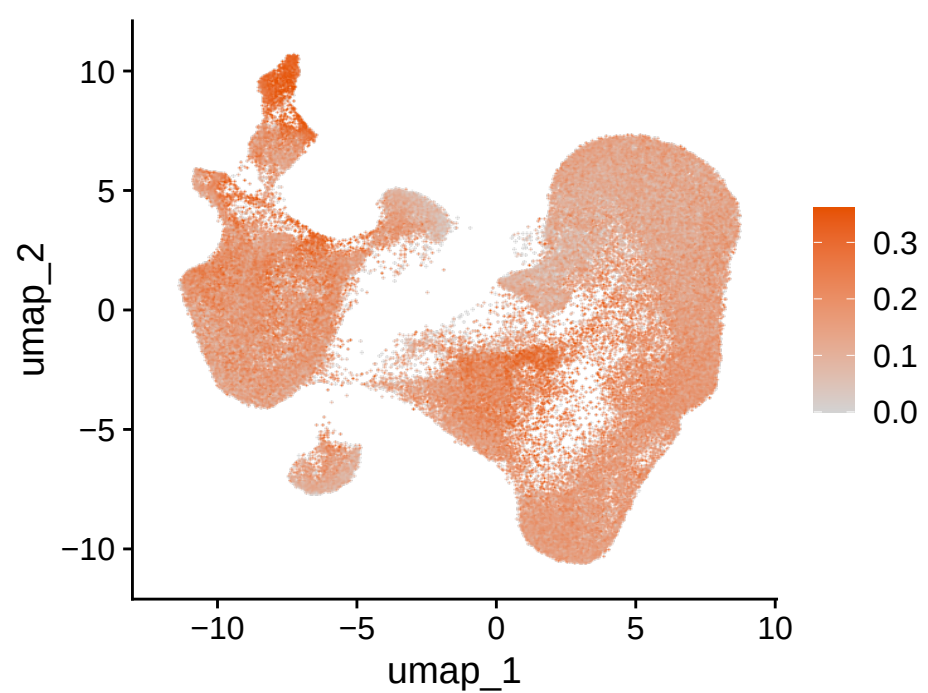
Chemokines
