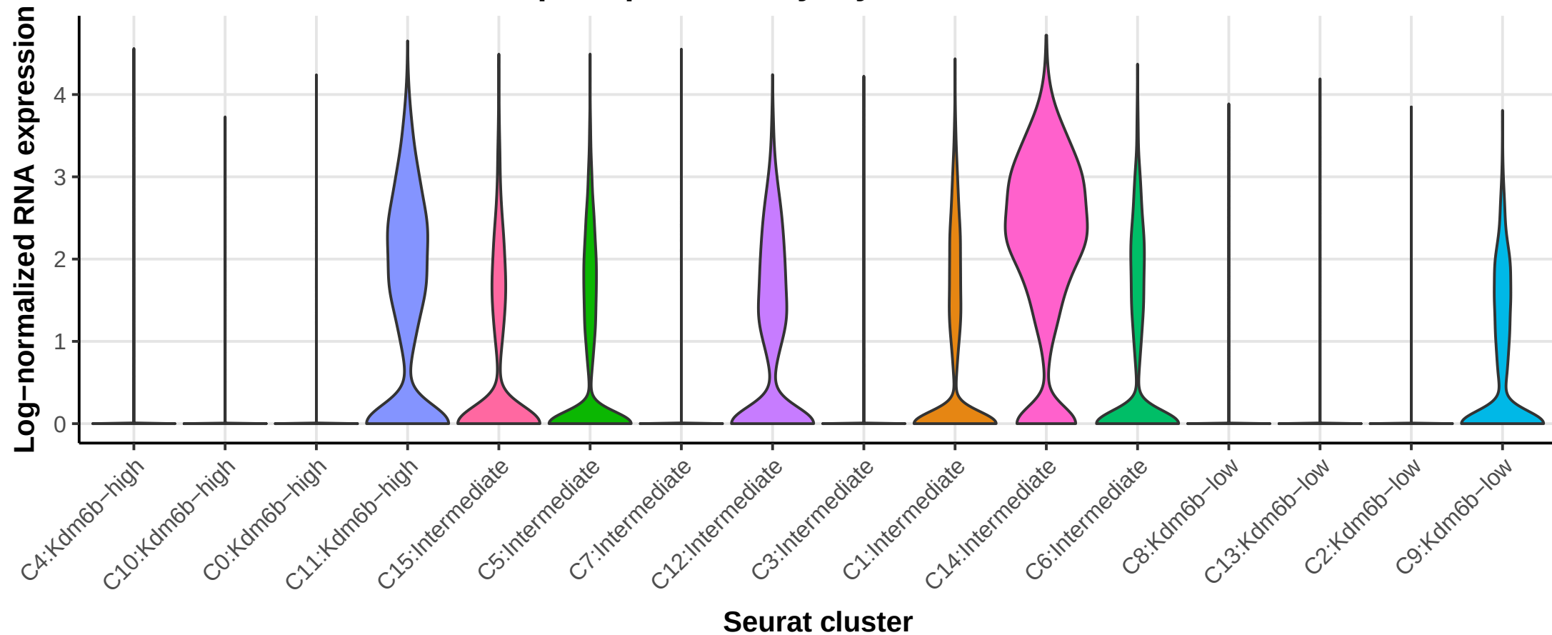
Tap1 expression by myeloid subcluster
