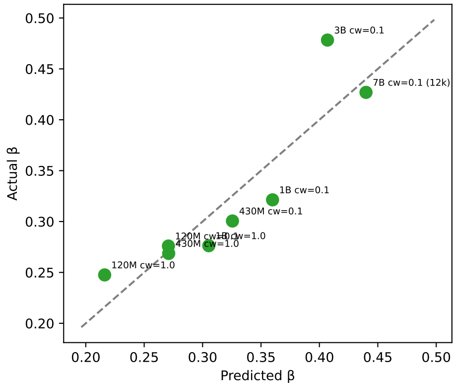
\beta regression ( R^2=0.809 )
