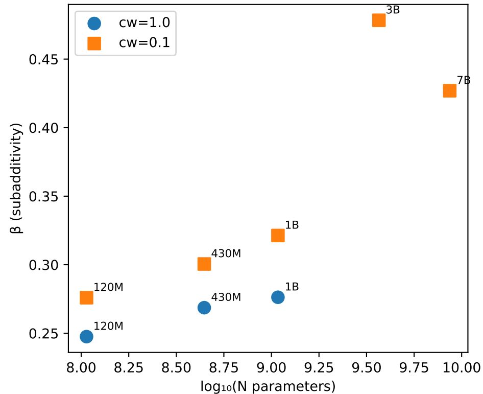
\beta vs scale, by consistency weight
