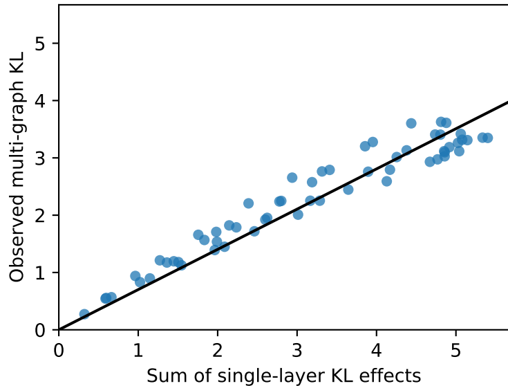
TinyStories ( \alpha=0.70 )
