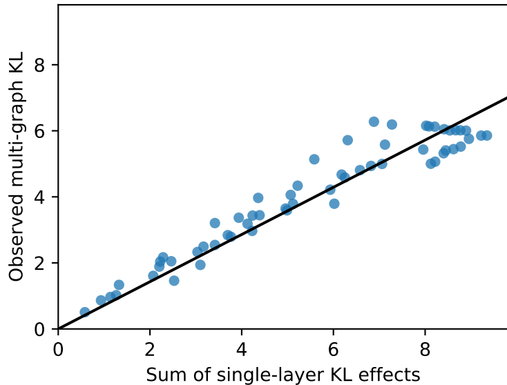
ClimbMix ( \alpha=0.71 )
