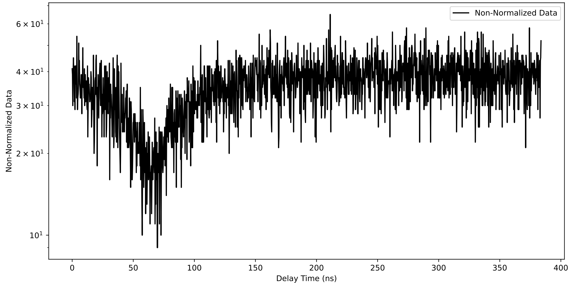
Non-Normalized Plot of Data
