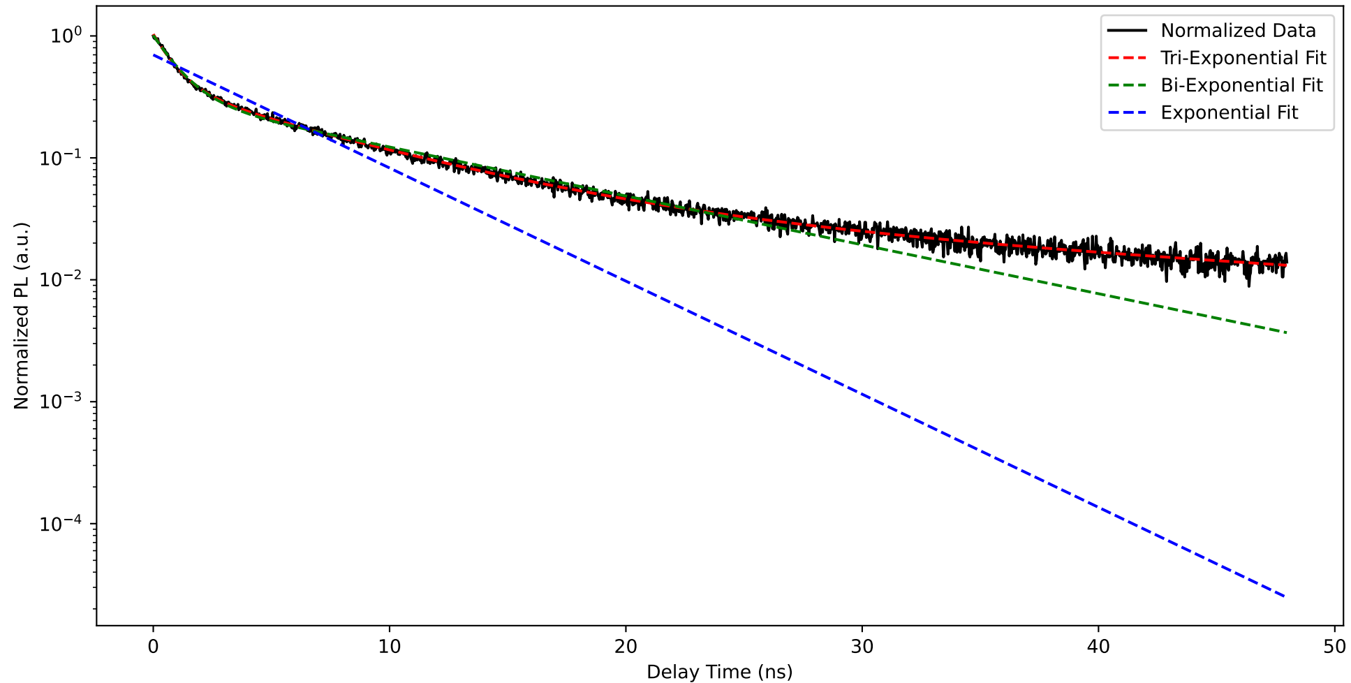
Comparison of Fits for Fluorescence Decay Data
