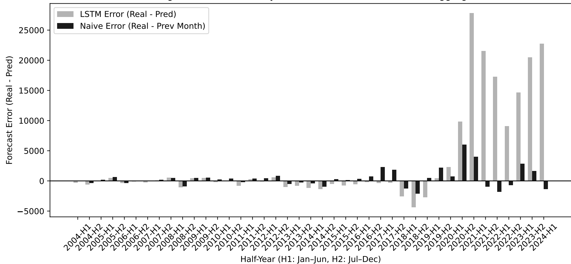
Samsung Electronics - 30-Day Ahead Forecast Error (Half-Year Aggregated)
