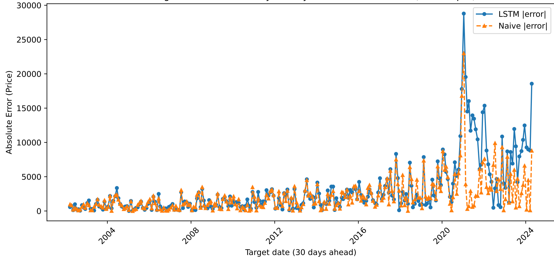
Samsung Electronics - Monthly 30-Day Ahead Absolute Error (OHLC input)
