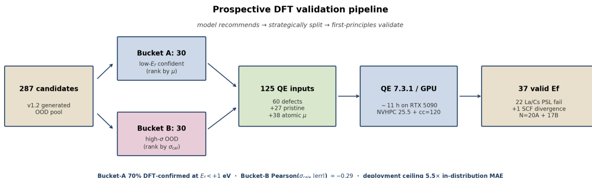
Figure 3: The prospective DFT validation pipeline: 287 model-generated OOD candidates are strategically split into 30 “low- E_f confident” (rank by \mu ) and 30 “high- \sigma OOD” (rank by \sigma_{cal} ) candidates with a 4-per-host diversity cap; the 60 selected candidates plus 27 pristine-host references plus 38 isolated-atom \mu references give 125 PBE PW SCF runs in Quantum ESPRESSO 7.3.1 with NVHPC 25.5 (CUDA 12.9, cc=120) on a single RTX 5090 in \sim 11 h wall. Of the 60 defect runs, 22 La/Cs candidates are rejected by a known PSL/PAW augmentation- l_{\max} incompatibility and one Sc@WTe 2 run fails SCF convergence, yielding N = 37 valid defect formation energies for the analysis below.
