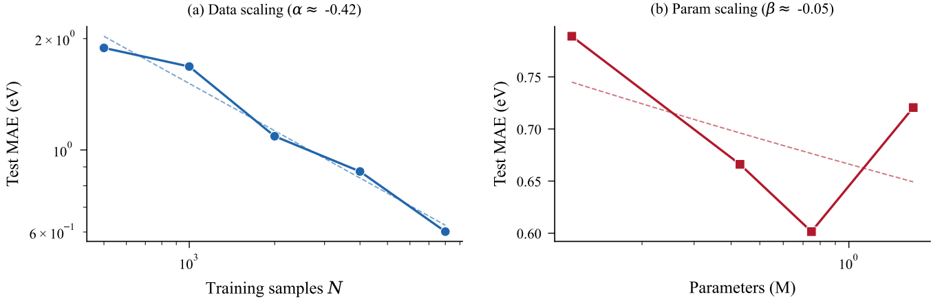
FIG. 8. Scaling analysis from abbreviated 30-epoch training runs. (a) Data scaling at fixed model size ( d = 128 ): power-law exponent \alpha \approx -0.4 indicates strong data dependence. (b) Parameter scaling at fixed data ( N = 8,000 ): \beta is near zero, showing negligible improvement from larger models. Both panels confirm that data, not capacity, is the bottleneck in the N \sim 10^4 regime.
