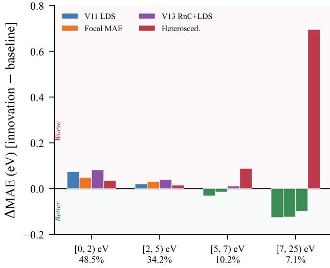
FIG. 7. Per-range MAE decomposition explaining why auxiliary losses fail. LDS and focal MAE sacrifice accuracy on the dominant [0, 2) eV range (48.5% of data) for marginal gains at the tail. Heteroscedastic uncertainty degrades all ranges through capacity competition.
