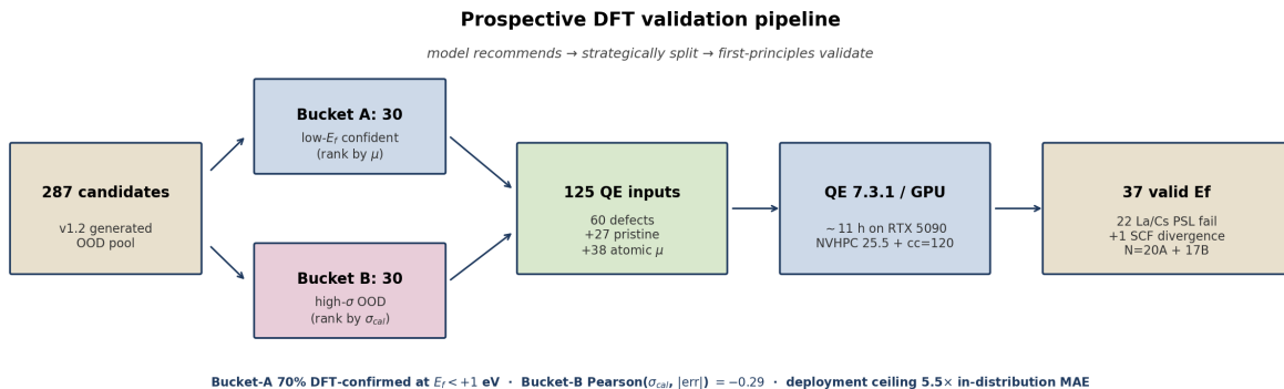
Figure 3: The prospective DFT validation pipeline: 287 model-generated OOD candidates are strategically split into 30 “low- E_f confident” (rank by \mu ) and 30 “high- \sigma OOD” (rank by \sigma_{\text{cal}} ) candidates with a 4-per-host diversity cap; the 60 selected candidates plus 27 pristine-host references plus 38 isolated-atom \mu references give 125 PBE PW SCF runs in Quantum ESPRESSO 7.3.1 with NVHPC 25.5 (CUDA 12.9, cc=120) on a single RTX 5090 in \sim 11 h wall. Of the 60 defect runs, 22 La/Cs candidates are rejected by a known PSL/PAW augmentation- l_{\text{max}} incompatibility and one \text{Sc@WTe}_2 run fails SCF convergence, yielding N = 37 valid defect formation energies for the analysis below.
