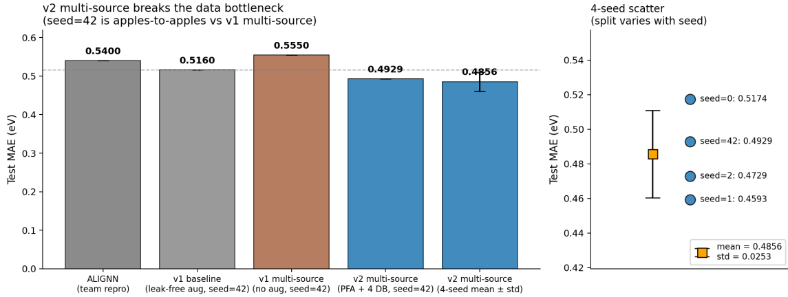
Figure 2: Multi-source progression. Left: bar comparison from ALIGNN through v1 baseline to v1 multi-source, PERIDEFT seed=42, and the PERIDEFT 4-seed mean. Right: per-seed scatter, showing all four seeds beat the v1 multi-source reference (dotted line) and three of four also beat the v1 leak-free single-source baseline (dashed line).
