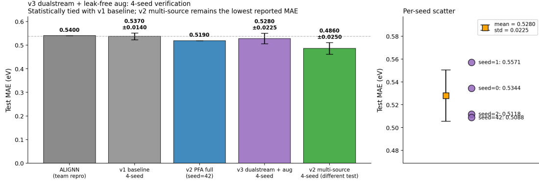
Figure 5: Dual-stream verification. Left: test MAE bars comparing ALIGNN, v1 baseline (4-seed), v2 PFA full (single seed), v3 dual-stream + aug (4-seed mean \pm std), and PERIDEFT (4-seed mean \pm std, on the multi-source split). Right: per-seed dual-stream scatter, with the orange marker indicating mean \pm standard deviation.
