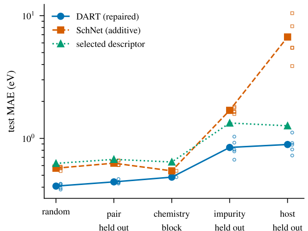
FIG. 5. Test MAE across the five transfer regimes for the repaired defect-centered model, the additive-readout SchNet baseline, and the validation-selected descriptor model (log scale). Small open markers show individual folds where five folds exist.
