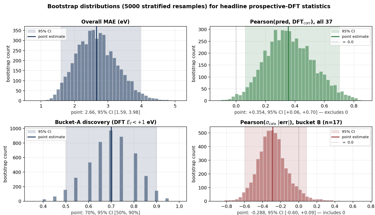
Figure 7: Bootstrap distributions (5 000 stratified-by-bucket resamples, seed 42) for the four headline statistics of the prospective DFT subsection. Solid vertical line: full-data point estimate. Shaded band: 95% percentile CI. Dotted grey line: zero reference. The overall predicted-vs-DFT Pearson correlation (top right) and the bucket-A discovery rate (bottom left) have CIs that exclude their respective null hypotheses (Pearson > 0 at p \approx 0.025 ; discovery > 0.18 pool base-rate well below the lower CI bound). The bucket-B within-bucket Pearson( \sigma_{\text{cal}} , |\text{err}| ) (bottom right) has a 95% CI that weakly straddles zero, motivating the conservative “deployment caveat” framing in the text.
