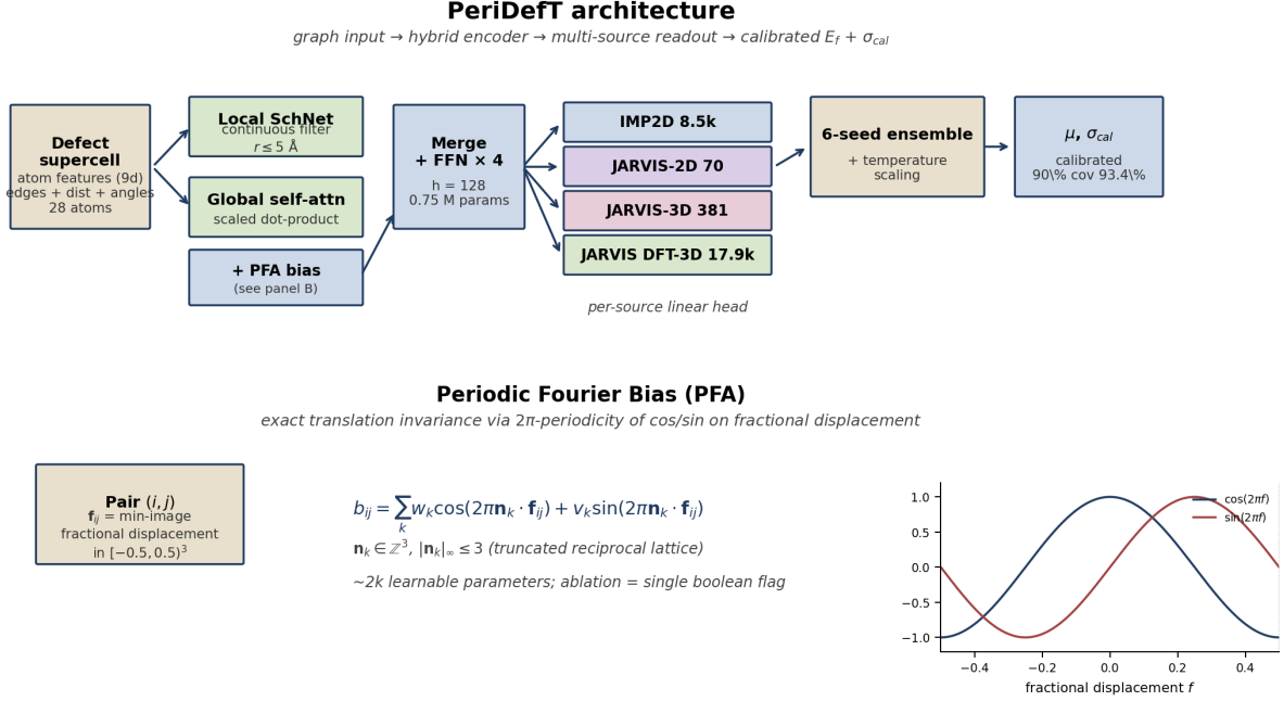
Figure 1: PERIDEFT architecture overview. Top: the data flow from a 28-atom defect supercell through the hybrid encoder to the four per-source readout heads, into the 6-seed temperature-scaled ensemble. Bottom: the Periodic Fourier Bias (PFA) on minimum-image fractional displacement \mathbf{f}_{ij} \in [-0.5, 0.5]^3 . PFA’s exact translation invariance follows from the 2\pi -periodicity of cos/sin on \mathbf{f}_{ij} (right inset); the ablation cost is a single boolean flag and the parameter overhead is \sim 2k .
