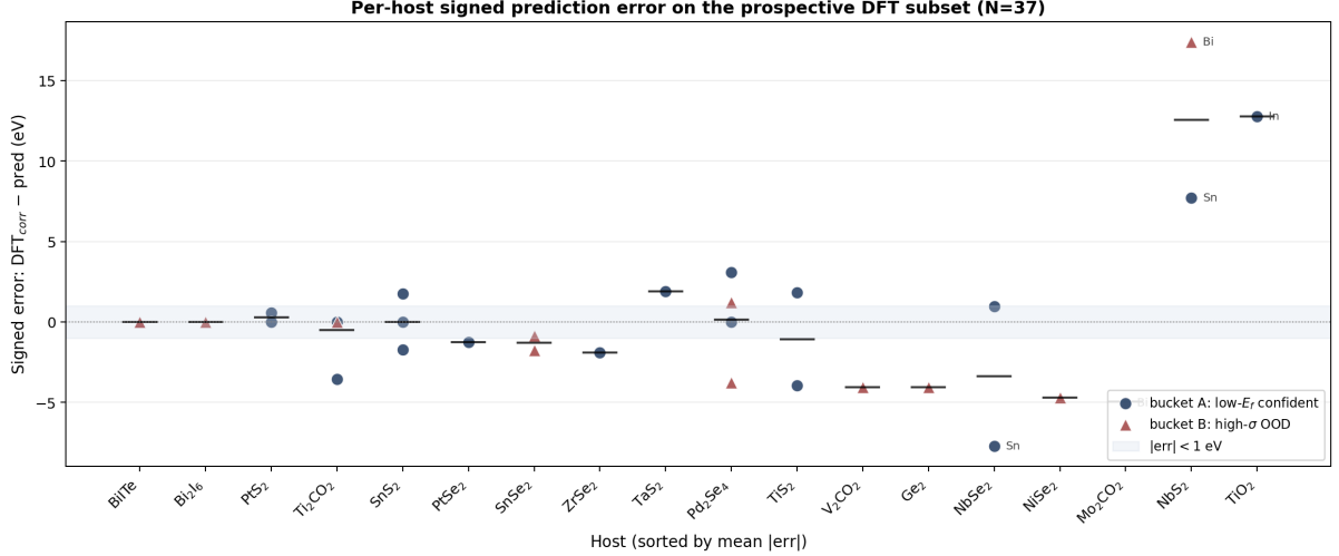
Figure 6: Per-host signed prediction error E_f^{\text{DFT,corr}} - E_f^{\text{pred}} on the 37-candidate prospective DFT subset, sorted left-to-right by mean |\text{err}| . Each marker is a single candidate (circle: bucket A; triangle: bucket B); the short horizontal tick is the per-host mean. The shaded band marks |\text{err}| < 1 eV. Most hosts (BiTe, Bi 2 I 6 , PtS 2 , Ti 2 CO 2 , SnS 2 , SnSe 2 , Pd 2 Se 4 ) fall within the band; a small number of host-dopant pairs — notably Bi@NbS 2 (B-bucket, +17.4 eV) and In@TiO 2 (A-bucket, +12.9 eV) — drive the heavy tail of the overall MAE distribution. Bucket A circles and bucket B triangles overlap in vertical extent, consistent with the within-bucket Pearson( \sigma_{\text{cal}} , |\text{err}| ) result.
