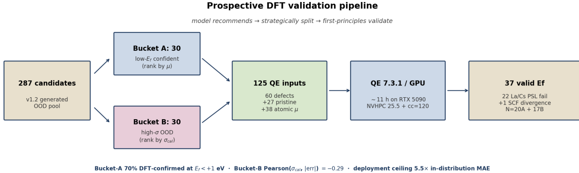
Figure 4: The prospective DFT validation pipeline: 287 model-generated OOD candidates are strategically split into 30 “low- E_f confident” (rank by \mu ) and 30 “high- \sigma OOD” (rank by \sigma_{cal} ) candidates with a 4-per-host diversity cap; the 60 selected candidates plus 27 pristine-host references plus 38 isolated-atom \mu references give 125 PBE PW SCF runs in Quantum ESPRESSO 7.3.1 with NVHPC 25.5 (CUDA 12.9, cc=120) on a single RTX 5090 in \sim 11 h wall. Of the 60 defect runs, 22 La/Cs candidates are rejected by a known PSL/PAW augmentation- l_{max} incompatibility and one Sc@WTe 2 run fails SCF convergence, yielding N = 37 valid defect formation energies for the analysis below.
