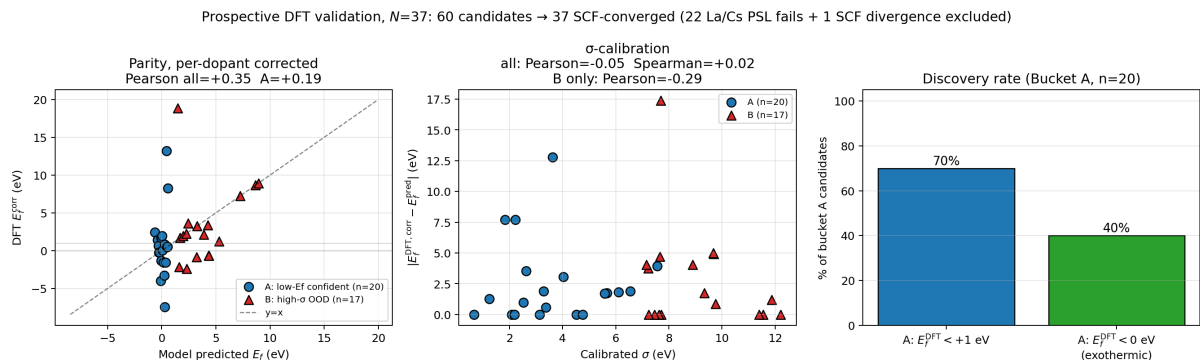
Figure 5: Prospective DFT validation on 37 SCF-converged model-recommended candidates (60 originally selected; 22 La/Cs candidates excluded due to PSL pseudopotential / pw.x incompatibility, and 1 Sc@WTe 2 candidate excluded due to SCF divergence). Left : parity of model predicted E_f vs DFT E_f after per-dopant chemical-potential offset correction, separated by selection bucket. Centre : calibrated uncertainty \sigma_{\text{cal}} vs absolute residual; the high- \sigma bucket-B subset (red triangles) shows a negative correlation between \sigma and |\text{error}| . Right : discovery rate within bucket A. The 70% hit rate at E_f < 1 eV is the primary deployment claim.
