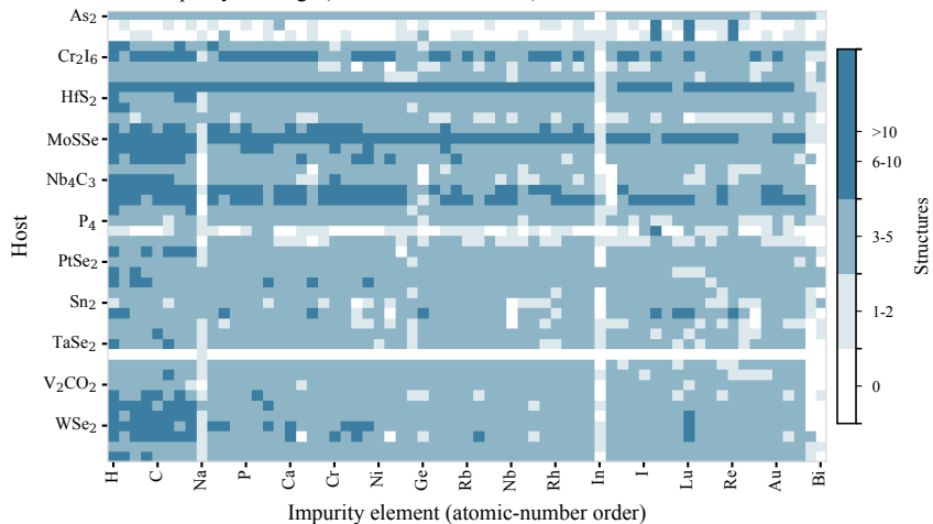
(c) Host-impurity coverage (44 hosts x 65 elements)
