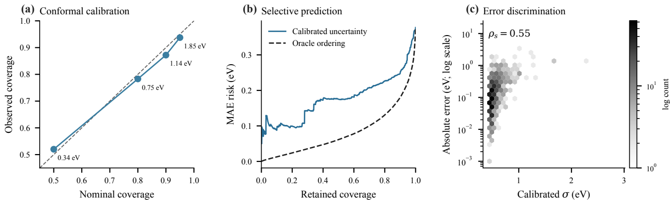
FIG. 5. Internal uncertainty evaluation on the dedicated ensemble split. (a) Nominal versus observed split-conformal coverage; annotations give mean interval widths. (b) MAE risk as increasingly uncertain predictions are rejected, compared with oracle ordering by realized error. (c) Calibrated standard deviation versus absolute error on the dedicated test partition.
