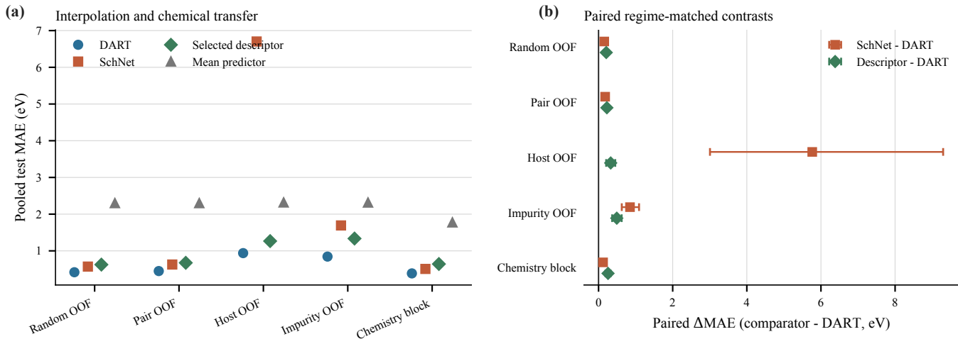
FIG. 3. Interpolation and chemical-transfer evaluation. (a) Pooled test MAE for DART, periodic SchNet, a descriptor family selected independently inside each split using its validation data, and a training-target mean predictor. (b) Paired differences in absolute error relative to DART with 95% bootstrap intervals using the regime-matched resampling units defined in Sec. III A. Positive values favor DART.
