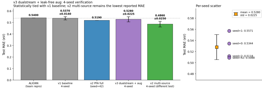
Figure 2: Dual-stream verification. Left: test MAE bars comparing ALIGNN, v1 baseline (4-seed), v2 PFA full (single seed), v3 dual-stream + aug (4-seed mean \pm std), and PERIDEFT(4-seed mean \pm std, on the multi-source split). Right: per-seed dual-stream scatter, with the orange marker indicating mean \pm standard deviation.
