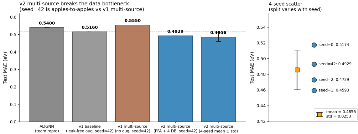
Figure 3: Multi-source progression. Left: bar comparison from ALIGNN through v1 baseline to v1 multi-source, PERIDEFT seed=42, and the PERIDEFT 4-seed mean. Right: per-seed scatter, showing all four seeds beat the v1 multi-source reference (dotted line) and three of four also beat the v1 leak-free single-source baseline (dashed line).
