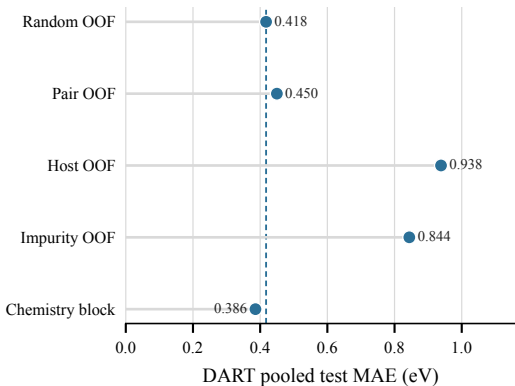
(a) DART error across transfer regimes
