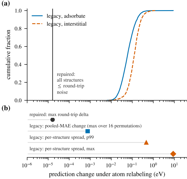
FIG. 6. Atom relabeling as a representation diagnostic. (a) Cumulative distribution of the per-structure prediction spread of the superseded (legacy) implementation across sixteen atom permutations, by incorporation class ( p_{99} = 0.46 eV, maximum 8.8 eV); under the repaired representation every structure reproduces its prediction to within the archived round-trip bound ( \leq 1.7 \times 10^{-5} eV, vertical line). (b) The same axis at aggregate level: the legacy pooled MAE changes by at most 8 \times 10^{-4} eV across permutations — four orders of magnitude below the largest single-structure spread — while individual relabelings flip 9–19 incorporation-class decisions and 76–102 site selections. Aggregate benchmarks are nearly blind to this defect.
