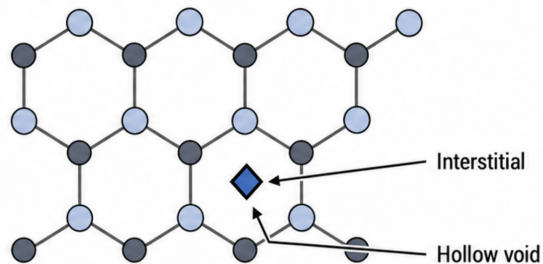
(b) Interstitial configuration
