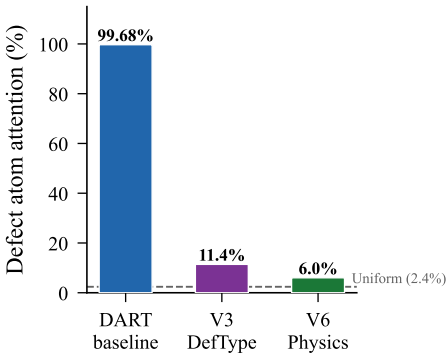
(a) Pooling attention
