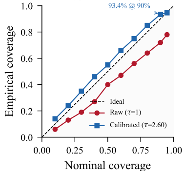
(c) UQ reliability
