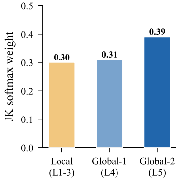
(b) V14 layer weights
