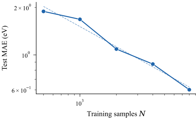
(a) Data scaling ( \alpha \approx -0.42 )
