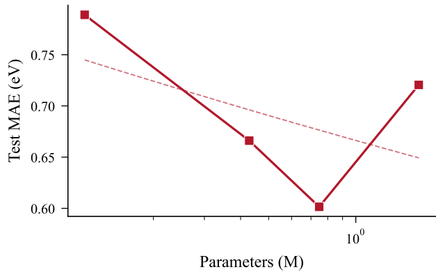
(b) Param scaling ( \beta \approx -0.05 )
