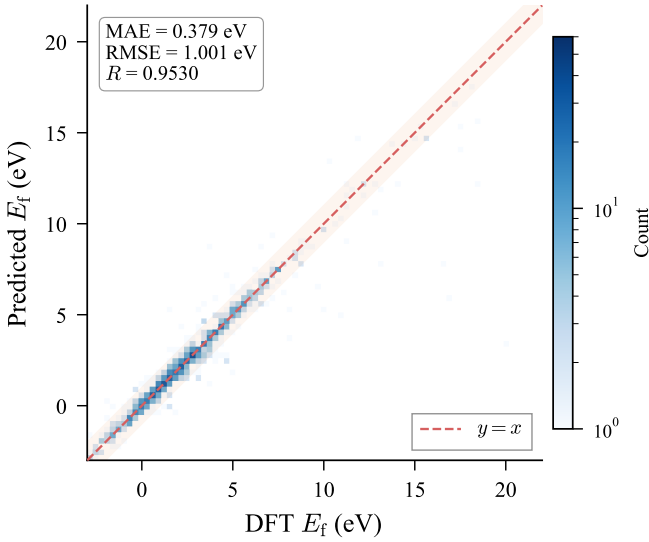
FIG. 4. Parity plot for the best single model (V4 MoE, 0.379 eV). Color intensity indicates sample density. The shaded band marks \pm 1 eV around perfect prediction.
