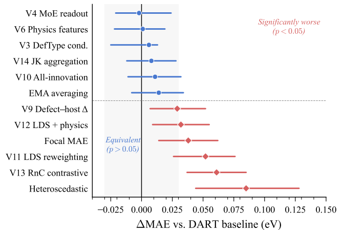
FIG. 1. Bootstrap confidence intervals for twelve innovation variants relative to the DART baseline. Blue circles: statistically equivalent ( p > 0.05 ). Red squares: significantly worse ( p < 0.05 ). Dashed line marks the \alpha = 0.05 significance boundary.
