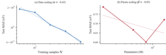
FIG. 6. Scaling analysis from abbreviated 30-epoch training runs. (a) Data scaling at fixed model size ( d = 128 ): power-law exponent \alpha \approx -0.4 indicates strong data dependence. (b) Parameter scaling at fixed data ( N = 8,000 ): \beta is near zero, showing negligible improvement from larger models. Both panels confirm that data, not capacity, is the bottleneck in the N \sim 10^4 regime.
