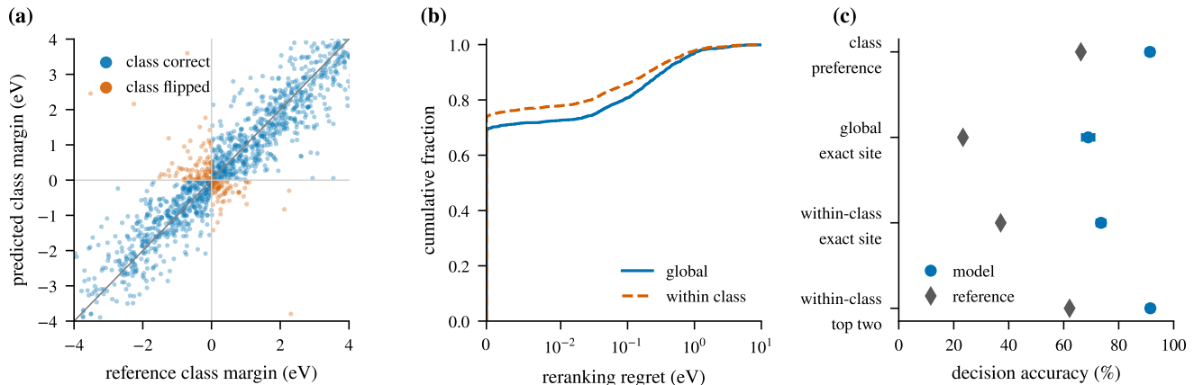
FIG. 5. Retrospective reranking of available DFT-relaxed IMP2D geometries from repaired pair-held-out predictions. (a) Predicted versus reference incorporation-class margins; flipped decisions (orange) cluster at small reference margins. (b) Empirical cumulative distributions of global and within-class reranking regret. (c) Host-impurity-pair cluster-bootstrap intervals for the four decision accuracies against their class-prior or uniform references (diamonds).
