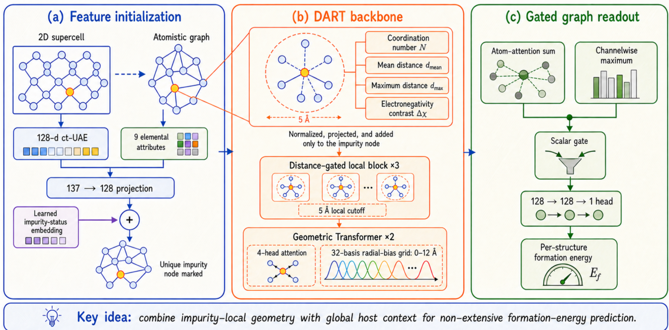
FIG. 1. Architecture of the Defect-Aware Radial Transformer (DART). (a) A fixed 128-dimensional ct-UAE vector and nine normalized elemental attributes are projected from 137 to 128 channels, after which a learned impurity-status embedding marks the unique impurity node. (b) A callout from that node enlarges its periodic 5-Å neighborhood and identifies the four defect-environment quantities: coordination number, mean and maximum neighbor distances, and electronegativity contrast. These quantities are normalized, projected, and added only at the impurity node before three 5-Å distance-gated local blocks and two four-head geometric Transformer blocks. The Transformer radial bias uses 32 basis functions spanning 0–12 Å. (c) A graph-dependent scalar gate fuses an atom-attention weighted sum and a channelwise maximum before a 128 → 128 → 1 head predicts one formation energy per structure. The small pictograms illustrate only the operations named in their enclosing boxes, and the bottom strip summarizes the same architecture-level design principle; neither introduces an additional model component. The schematic was edited with OpenAI GPT Image 2; the authors specified and verified its scientific content.
