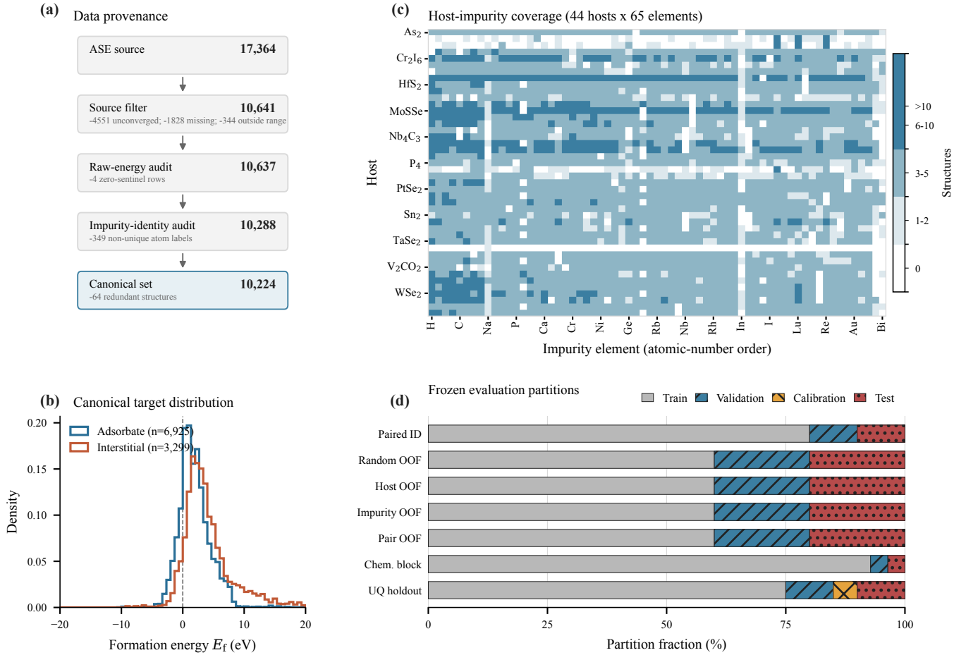
FIG. 3. Data provenance and evaluation protocol. (a) Sequential source filtering, raw-energy reconstruction audit, impurity-identity audit, and structure canonicalization. The final set excludes four rows with zero sentinels in a raw energy component, 349 rows without a unique impurity atom, and 64 redundant structures. (b) Formation-energy distributions for the two incorporation classes in the retained set. (c) Number of structures for each of 44 hosts and 65 impurity elements; white cells are unobserved combinations. (d) Train, validation, calibration, and test fractions for each evaluation regime. Bars for fivefold protocols show fold averages. All regimes cover the same 10,224 retained structures; the common 417-row exclusion set is omitted from the bars.
