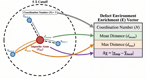
FIG. 4. Illustration of the defect-environment enrichment (E) module. Within the periodic 5-Å neighbor graph, four impurity-centered quantities—the neighbor count N , mean and maximum neighbor distances ( d_{\text{mean}} and d_{\text{max}} ), and the normalized Pauling-electronegativity contrast \Delta\chi = |\chi_{\text{imp}} - \langle\chi_{\text{nn}}\rangle| —form a four-component descriptor. The descriptor is normalized, projected to 128 channels, and added only to the impurity-node representation before local message passing. The N = 3 neighborhood shown is schematic.
