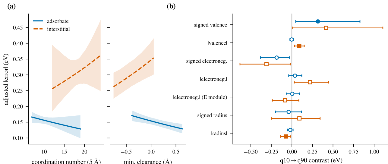
FIG. 6. Physical error map on repaired pair-held-out predictions. (a) Adjusted absolute-error profiles versus smooth coordination and post-relaxation clearance, by incorporation class, with pointwise intervals. (b) Chemistry-mismatch decile contrasts with pair-clustered intervals; filled markers pass the preregistered main-text gate, open markers do not.
