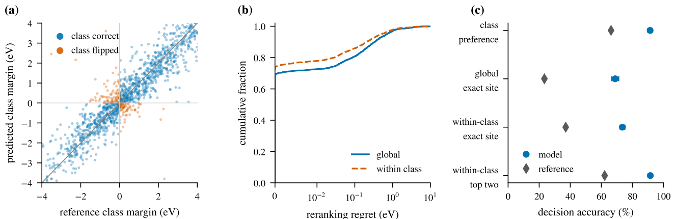
FIG. 8. Retrospective reranking of available DFT-relaxed IMP2D geometries from repaired pair-held-out predictions. (a) Predicted versus reference incorporation-class margins; flipped decisions (orange) cluster at small reference margins. (b) Empirical cumulative distributions of global and within-class reranking regret. (c) Host-impurity-pair cluster-bootstrap intervals for the four decision accuracies against their class-prior or uniform references (diamonds).
