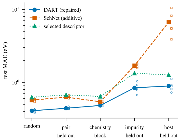
FIG. 5. Test MAE across the five transfer regimes for the repaired defect-centered model, the additive-readout SchNet baseline, and the validation-selected descriptor model (log scale). Small open markers show individual folds where five folds exist.
