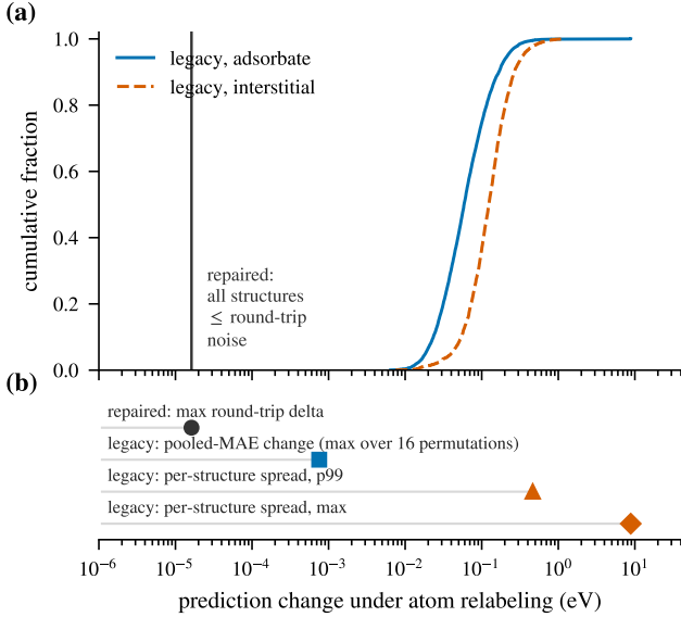
FIG. 9. Atom relabeling as a representation diagnostic. (a) Cumulative distribution of the per-structure prediction spread of the superseded (legacy) implementation across sixteen atom permutations, by incorporation class ( p_{99} = 0.46 eV, maximum 8.8 eV); under the repaired representation every structure reproduces its prediction to within the archived round-trip bound ( \leq 1.7 \times 10^{-5} eV, vertical line). (b) The same axis at aggregate level: the legacy pooled MAE changes by at most 8 \times 10^{-4} eV across permutations — four orders of magnitude below the largest single-structure spread — while individual relabelings flip 9–19 incorporation-class decisions and 76–102 site selections. Aggregate benchmarks are nearly blind to this defect.
