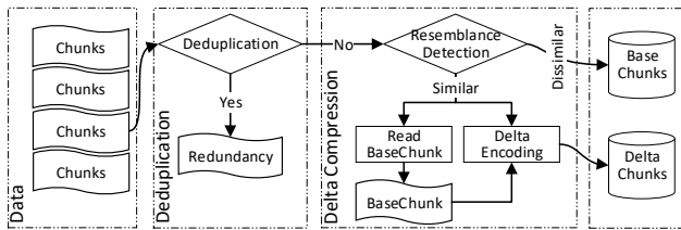
Fig. 13. General workflow of a prototype data reduction system.
