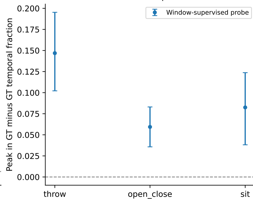
Pseudo: relative temporal evidence
